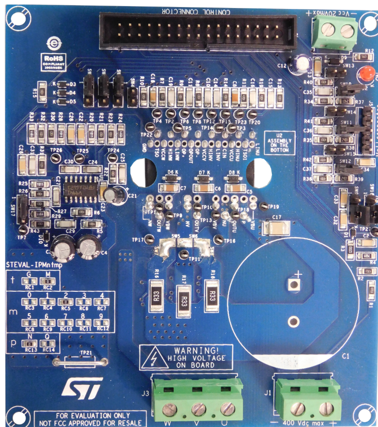
Figure 1. Motor control board (top view) based on SLLIMM-nano™ MOSFET
