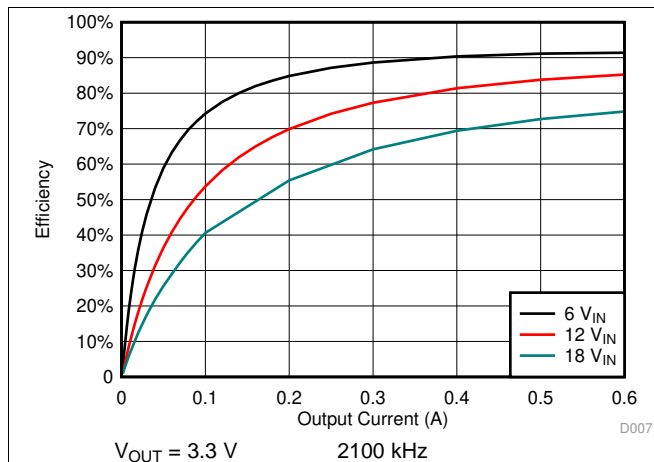
Figure 44. Efficiency
