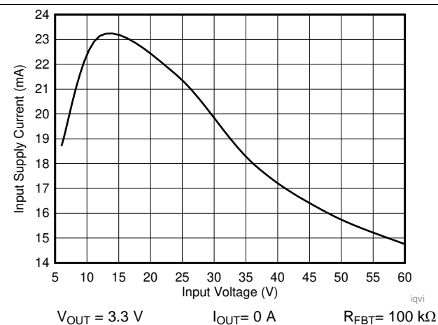
Figure 47. Input Supply Current
