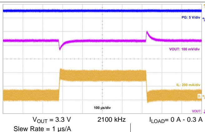
Figure 49. Load Transient
