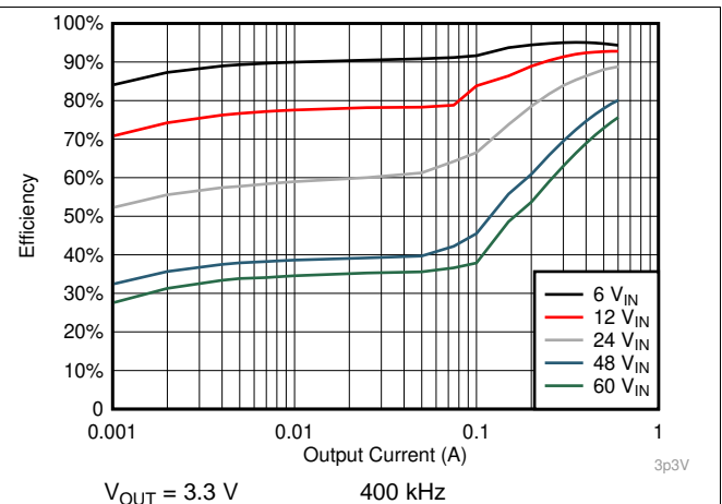
Figure 23. Efficiency
