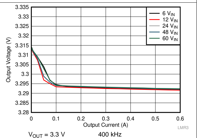
Figure 25. Load Regulation
