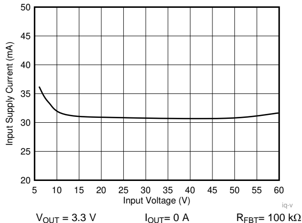
Figure 28. Input Supply Current
