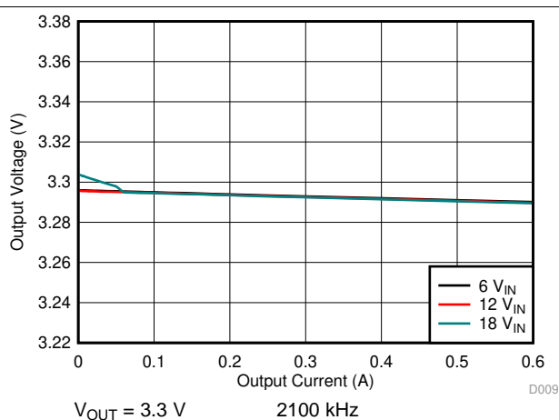
Figure 45. Load Regulation
