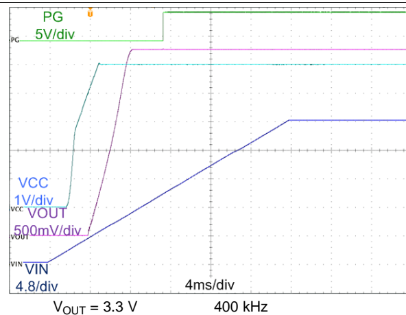
Figure 31. Start-Up Waveform
