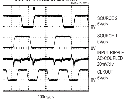
OUT-OF-PHASE OPERATION
