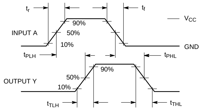
Figure 2. Switching Waveform
