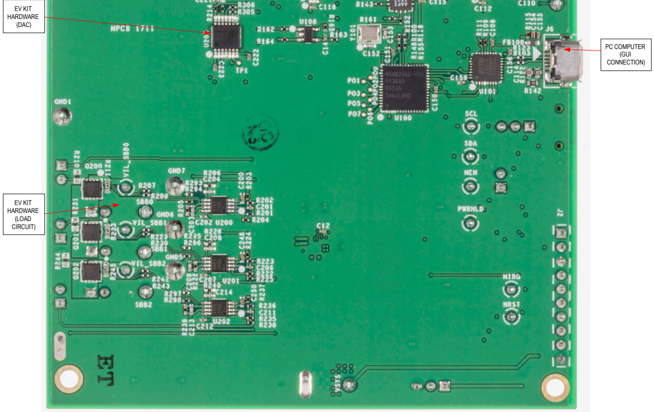
Figure 4. MAX77680/MAX77681 EV Kit Bottom View
