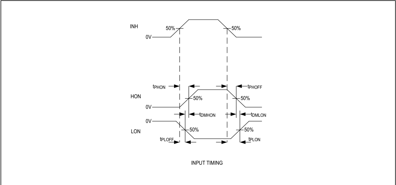
Figure 1. Timing Diagram
