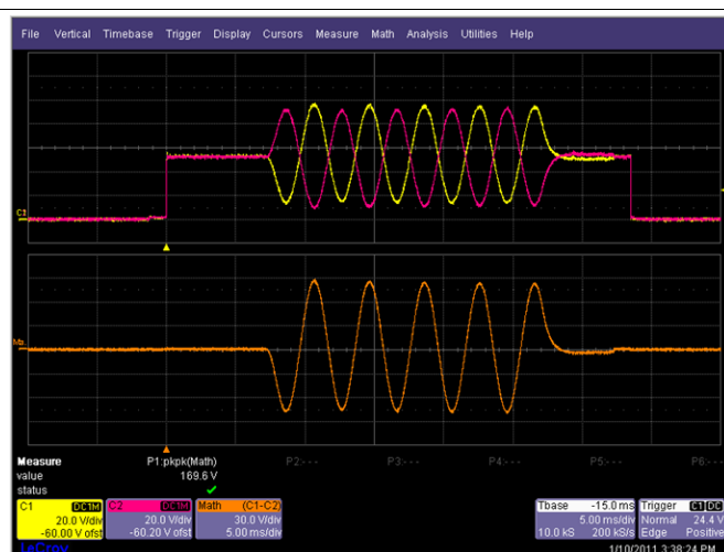
Figure 13. Second-Order, Differential Filter
