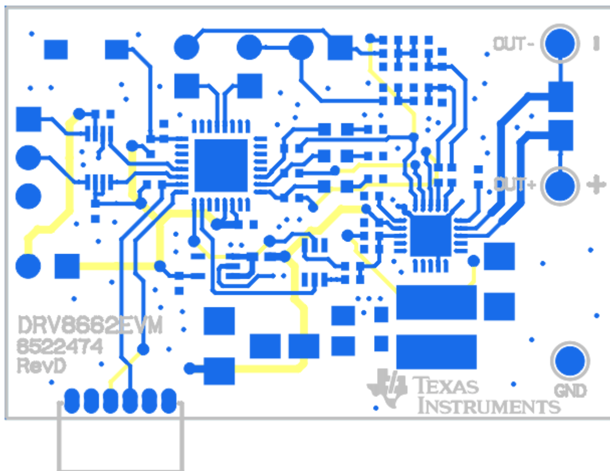
Figure 16. EVM Top X-Ray
