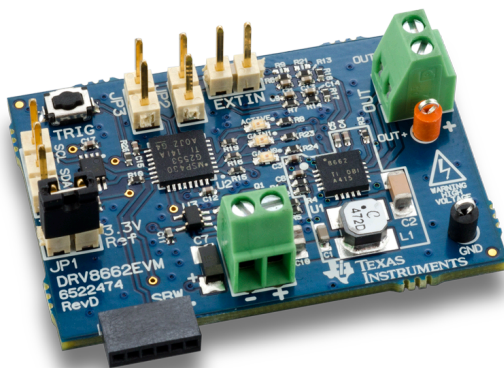
Figure 1. DRV8662EVM
