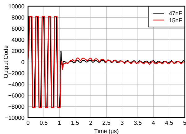
Figure 59. Overload Recovery Response vs. INM capacitor, V_{in} = 50 mVpp/100 \mu Vpp, Max Gain
