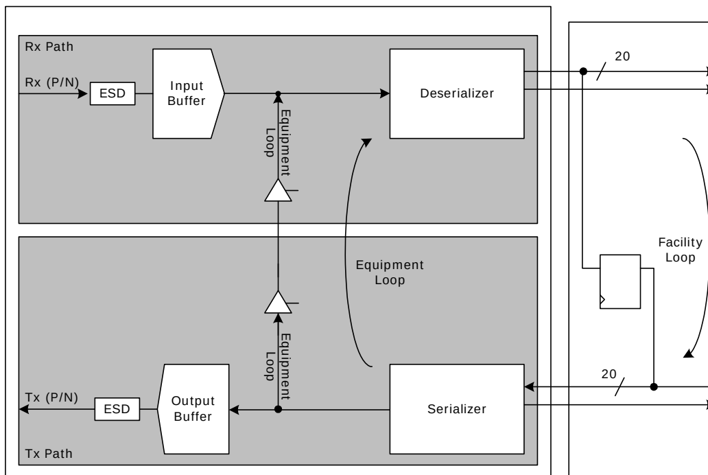
Figure 4 • SERDES Loopback
