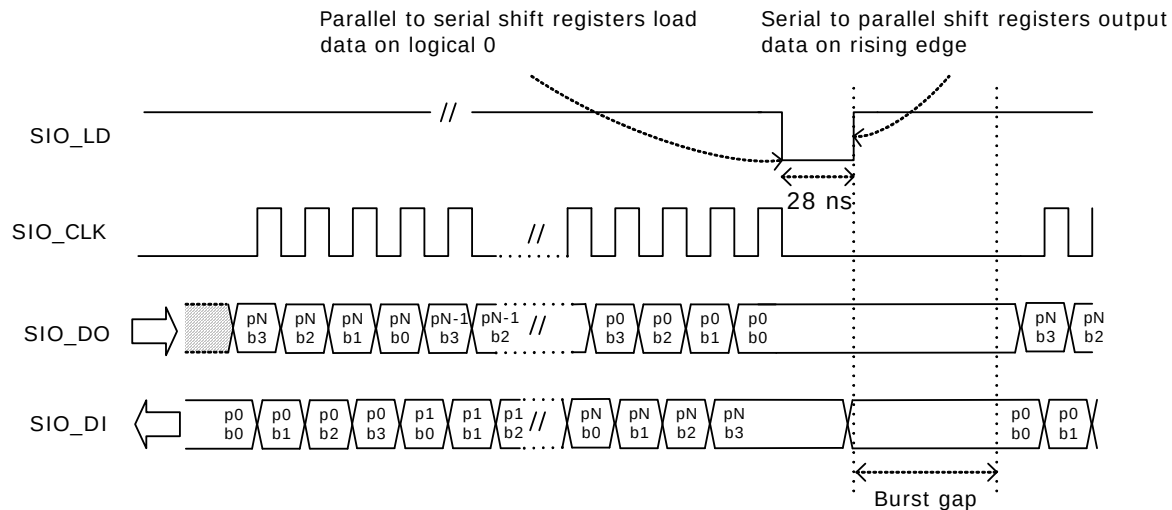
Figure 39 • SIO Timing
