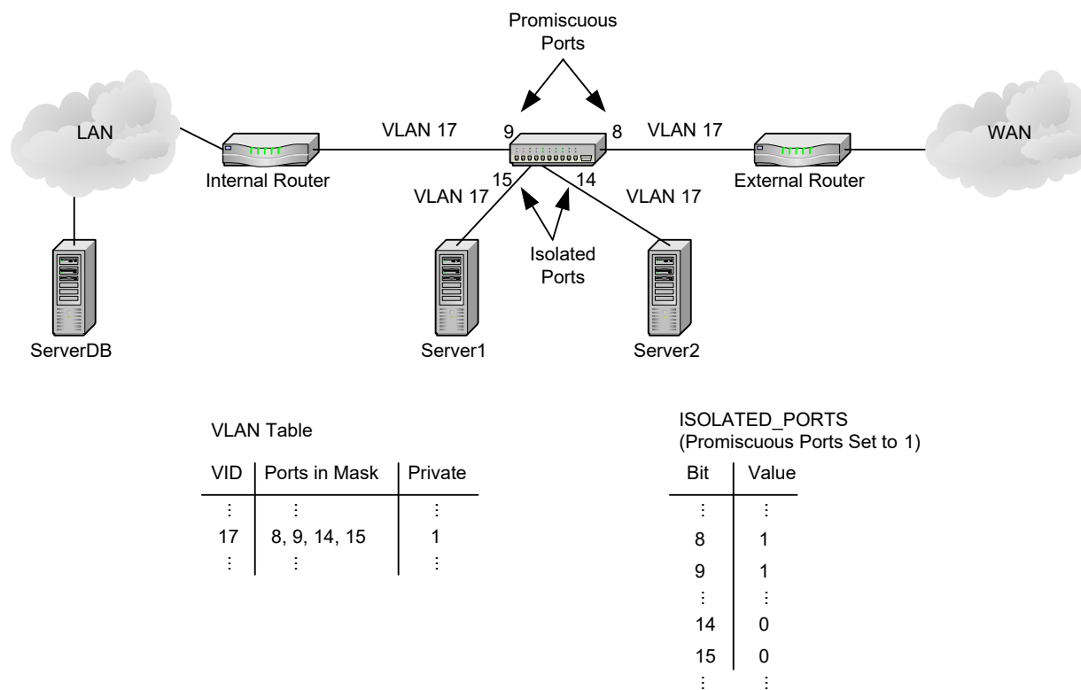
Figure 47 • DMZ Example for Private VLAN
