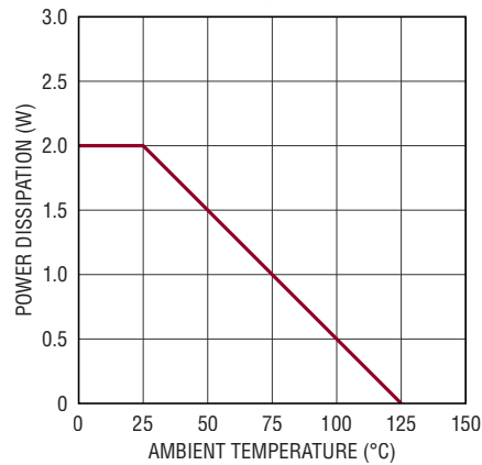
Thermal Derating
