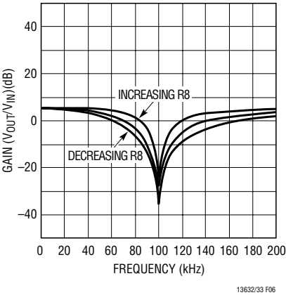
Figure 6. Frequency Response
