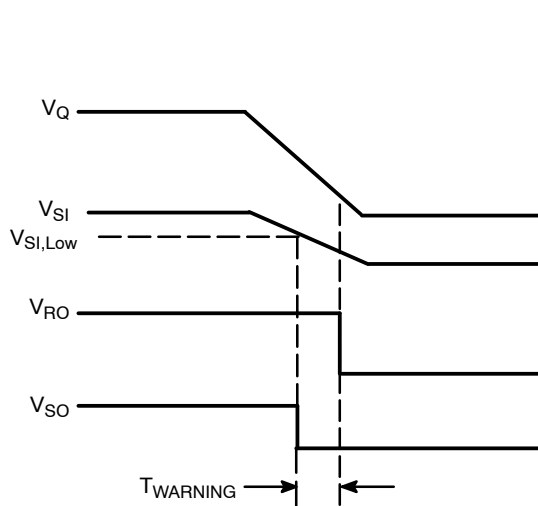
Figure 42. SO Warning Timing Waveform
