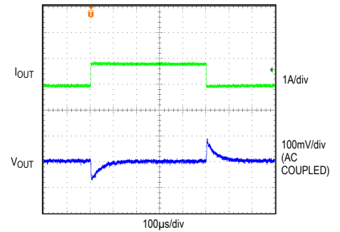
LOAD CURRENT TRANSIENT RESPONSE
