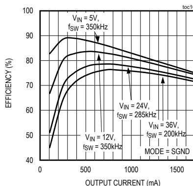
EFFICIENCY vs. OUTPUT CURRENT V OUT = 1.2V, PWM MODE
