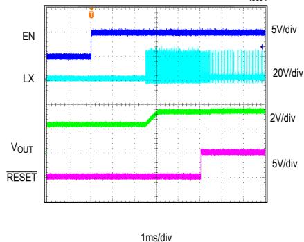
STARTUP WITH 2.5V PREBIAS
