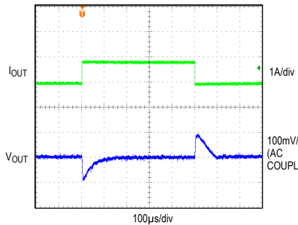
LOAD CURRENT TRANSIENT RESPONSE
