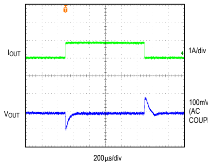
LOAD CURRENT TRANSIENT RESPONSE
