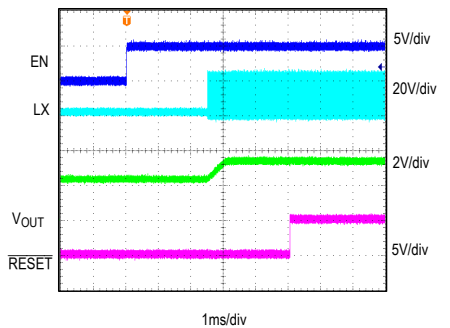
STARTUP WITH 2.5V PREBIAS
