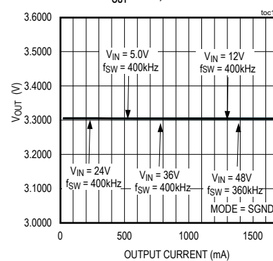
LOAD REGULATION V OUT = 3.3V, PWM MODE
