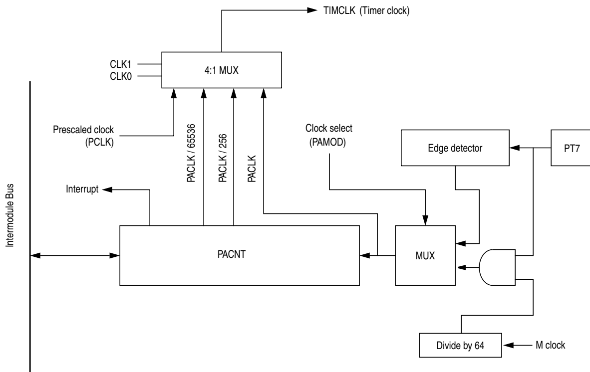
Figure 6-2. 16-Bit Pulse Accumulator Block Diagram
