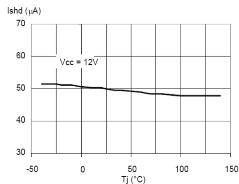
Figure 32. Shutdown current vs. junction temperature
