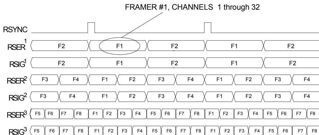
Figure 34-16. Receive IBO Frame Interleave Mode Timing
