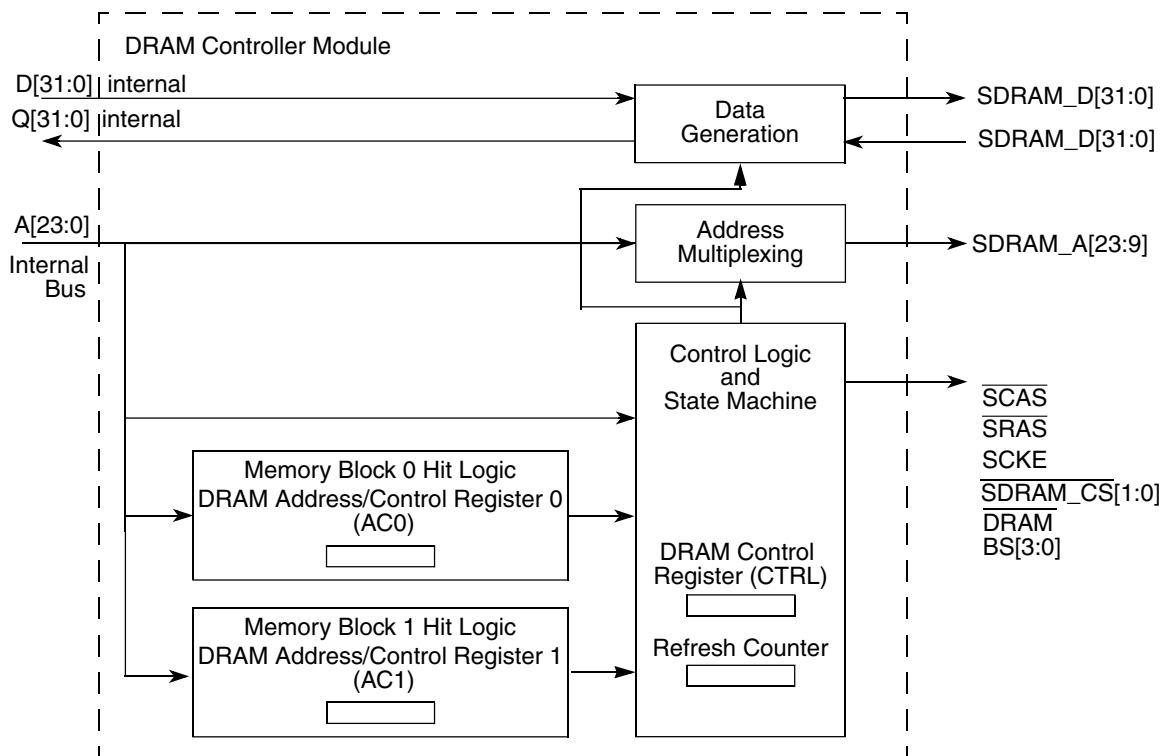
Figure 34-1. Block diagram
