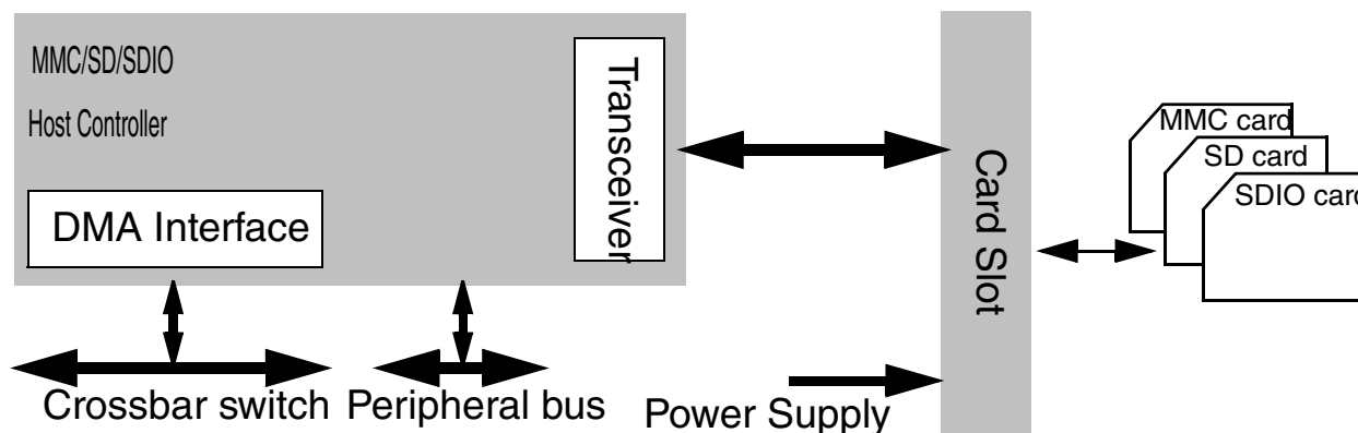
Figure 61-1. System connection of the SDHC
