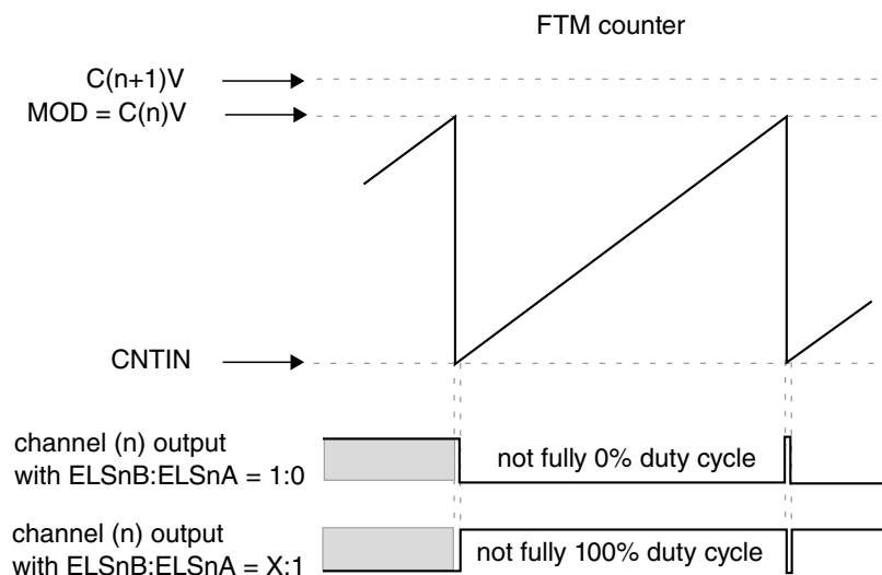
Figure 44-45. Channel (n) output if (C(n+1)V > MOD) and (CNTIN < C(n)V = MOD)
