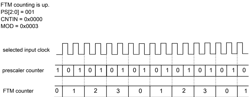
Figure 44-8. Example of the prescaler counter
