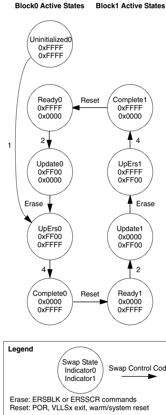
Figure 33-7. Valid Swap State Sequencing
