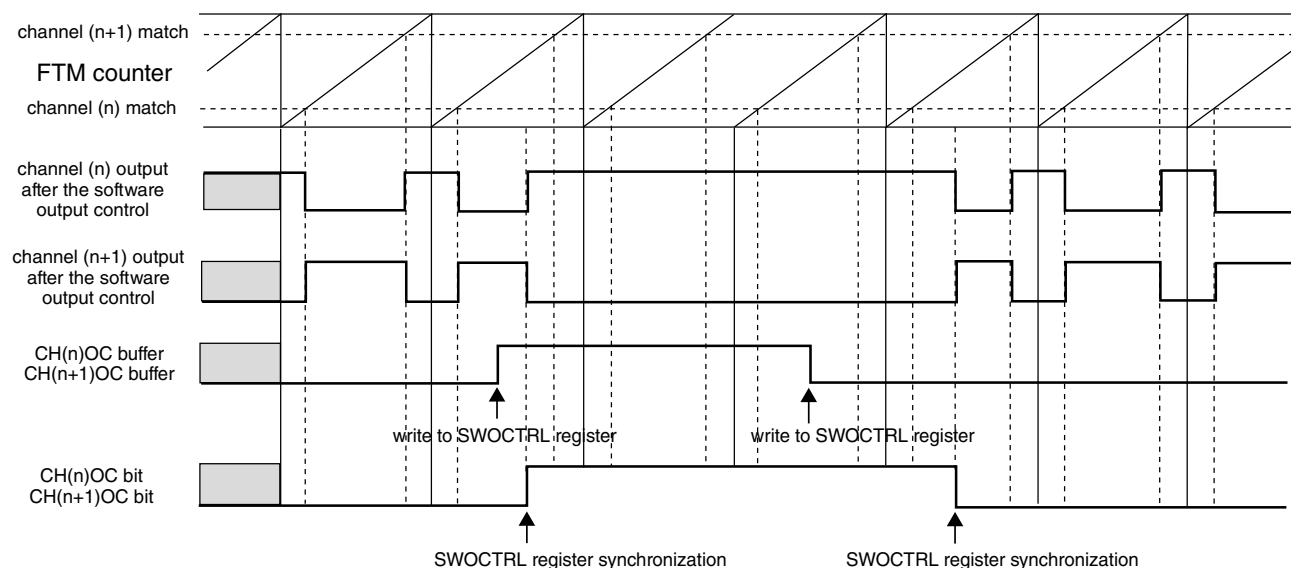
Figure 44-70. Example of software output control in Combine and Complementary mode
