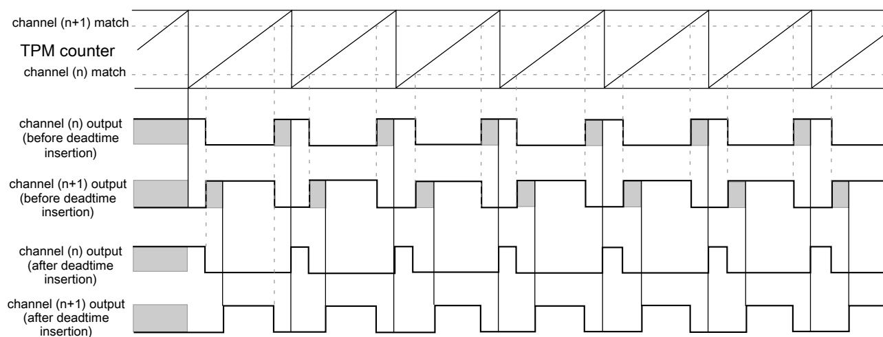
Figure 45-26. Deadtime insertion with ELSnB:ELSnA = 1:0 , POL(n) = 0 , and POL(n+1) = 1
