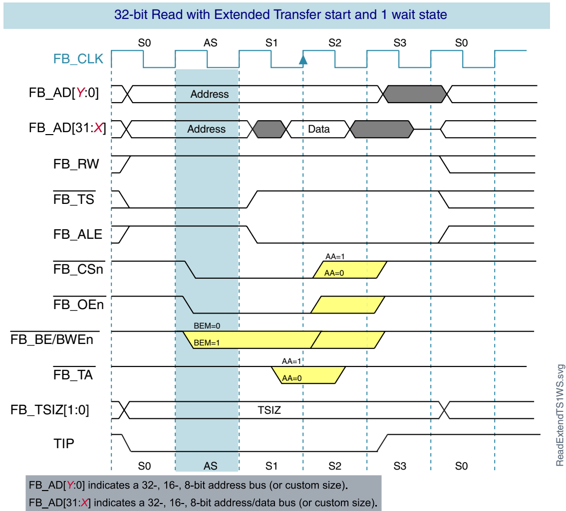
Figure 36-30. Read-Bus Cycle with CSCRn[EXTS] = 1 (One Wait State)
