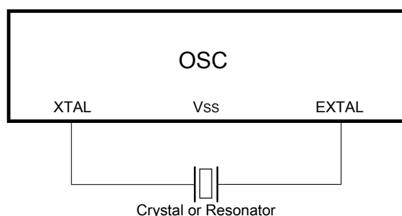
Figure 29-2. Crystal/Ceramic Resonator Connections - Connection 1
