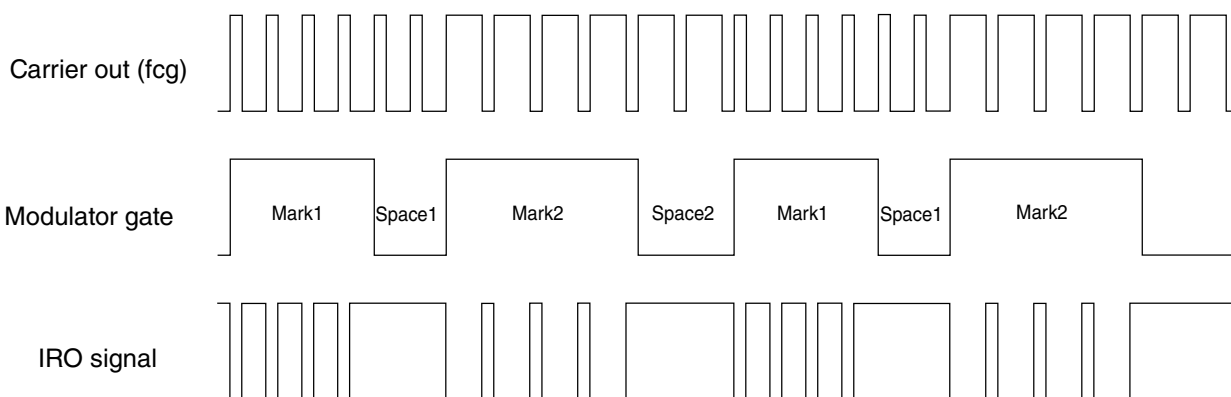
Figure 47-6. Example: CMT output in FSK mode
