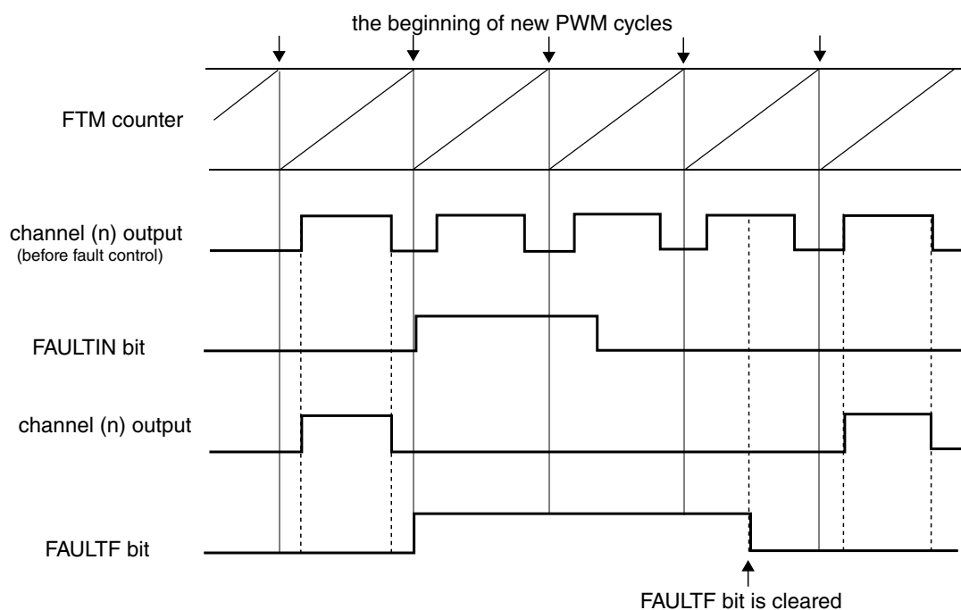
Figure 44-79. Fault control with manual fault clearing
