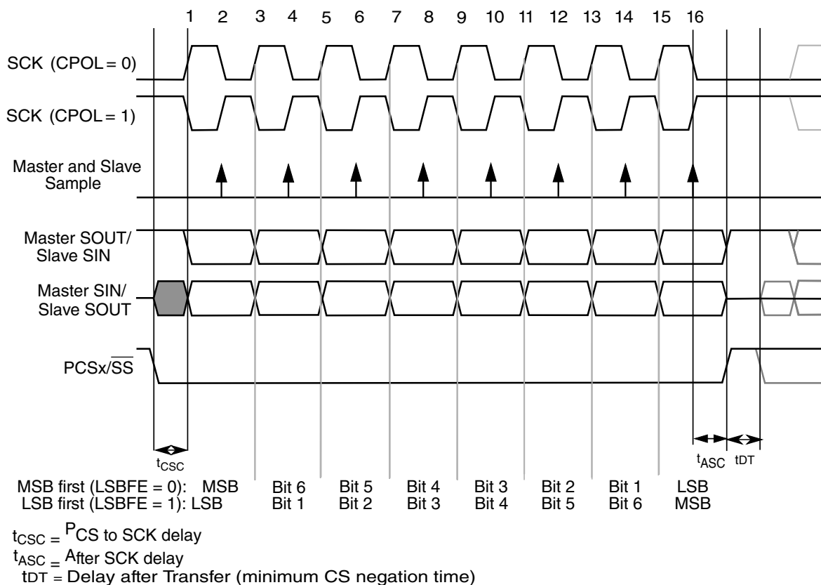
Figure 56-7. Module transfer timing diagram (MTFE=0, CPHA=1, FMSZ=8)
