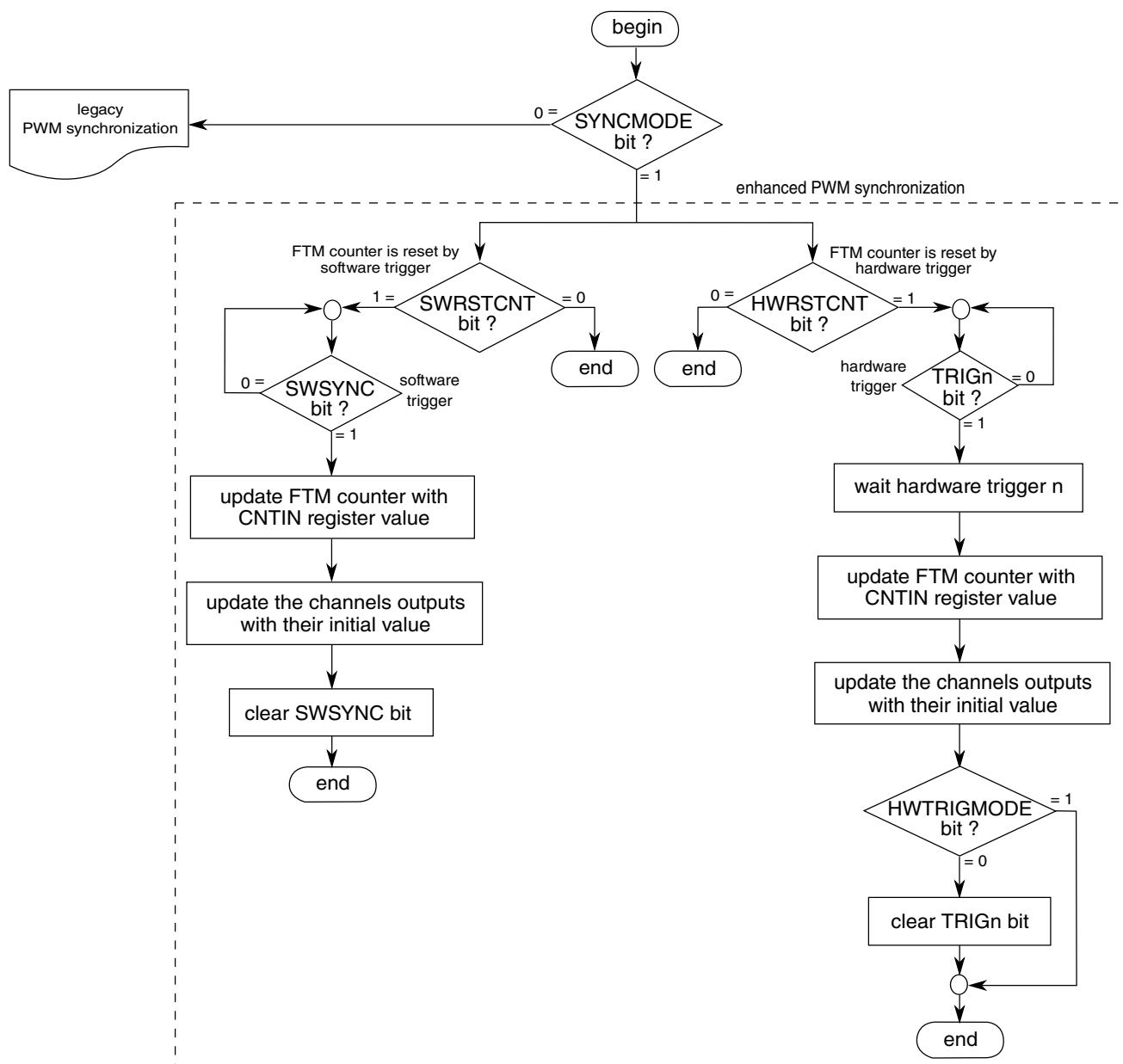
Figure 44-64. FTM counter synchronization flowchart
