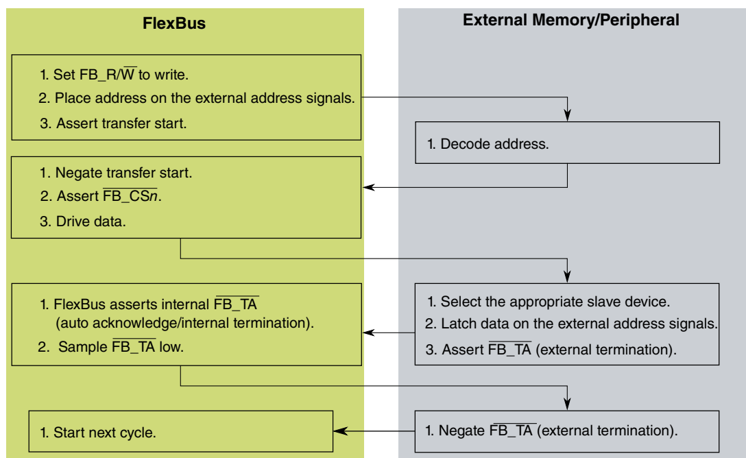
Figure 36-6. Write-Cycle Flowchart
