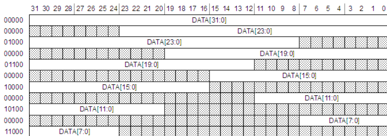
Figure 60-3. SAI first bit shifted, LSB first
