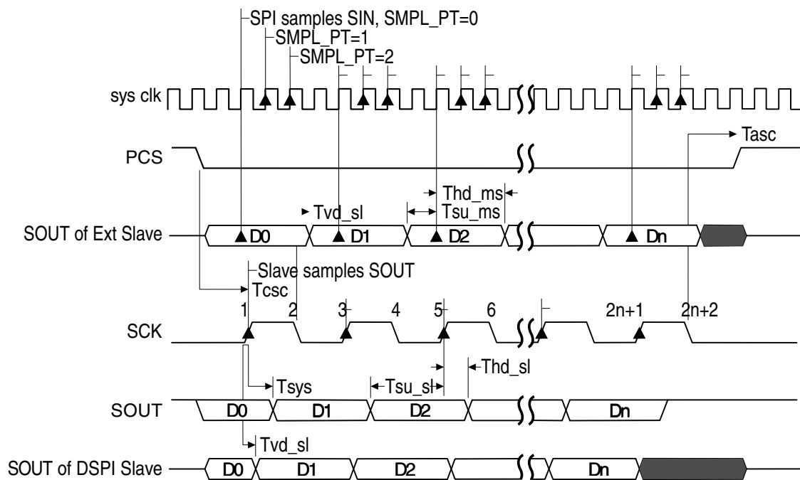
Figure 56-8. SPI Modified Transfer Format (MTFE=1, CPHA=0, f_{\text{sck}} = f_{\text{sys}}/4 )
