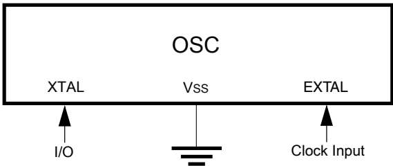
Figure 29-5. External Clock Connections
