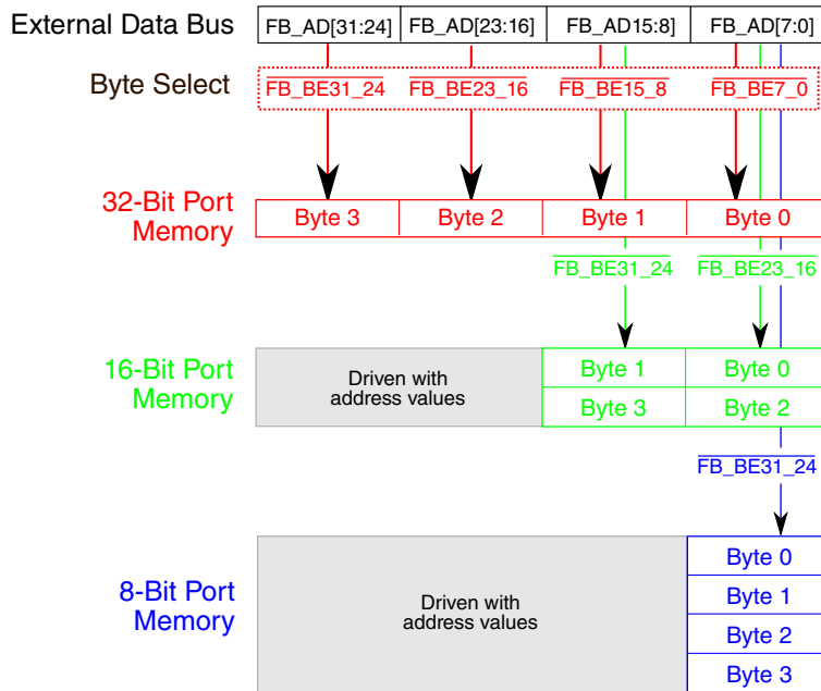
Figure 36-3. Connections for external memory port sizes (CSCRn[BLS] = 1)
