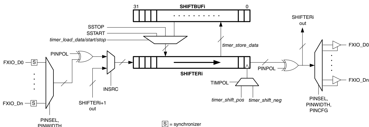
Figure 59-2. Shifter Microarchitecture
