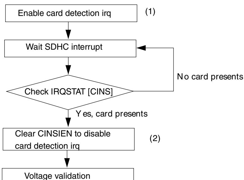
Figure 61-15. Flow diagram for card detection
