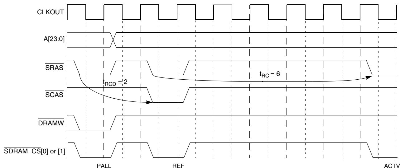
Figure 34-5. Auto-Refresh Operation
