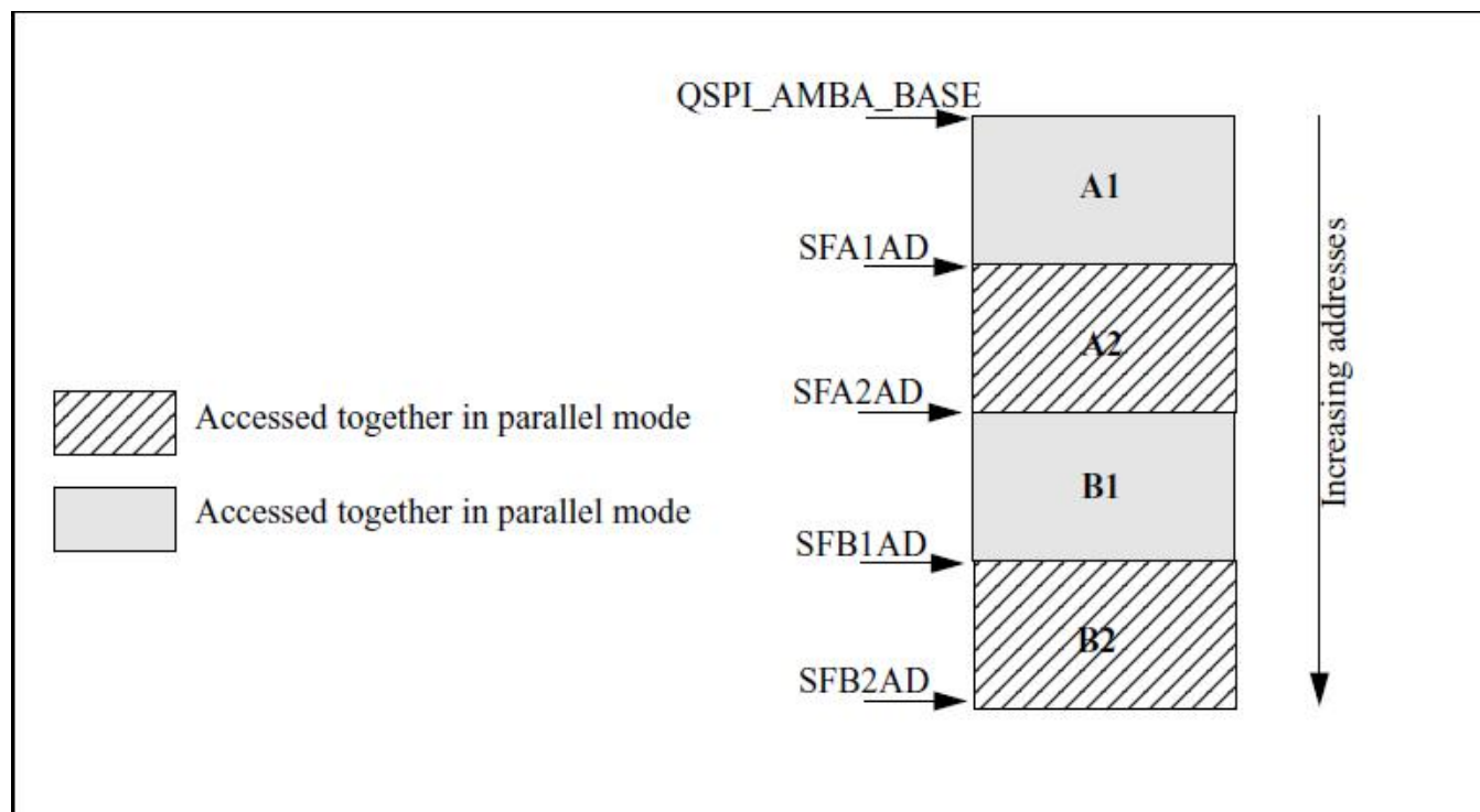
Figure 35-8. Flash addressing
