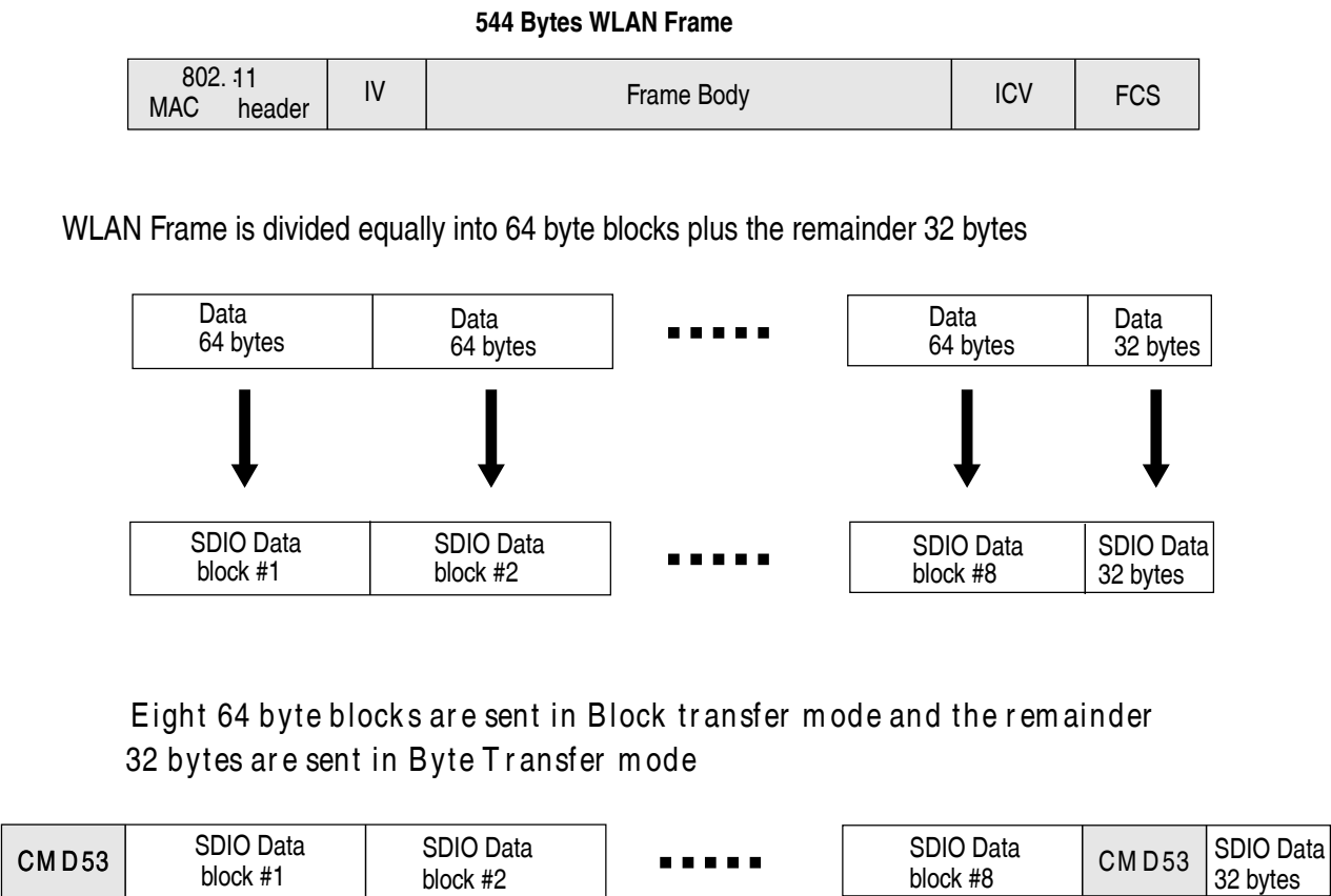
Figure 61-6. Example for dividing large data transfers
