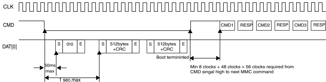
Figure 61-13. Multimediacard state diagram in Normal Boot mode
