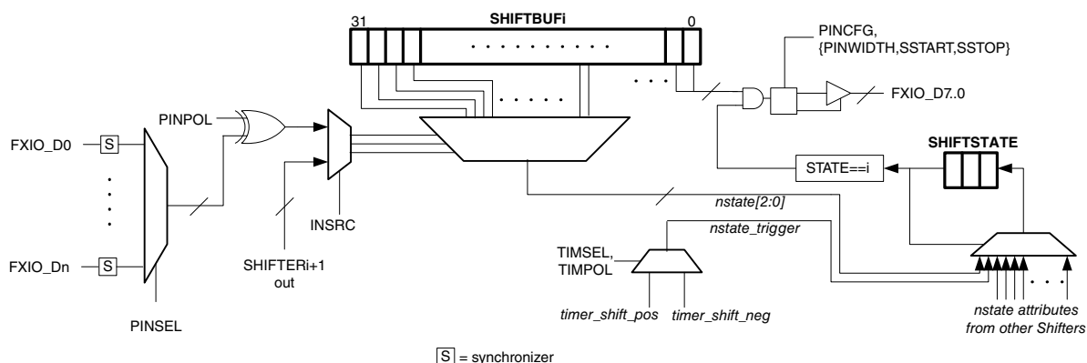
Figure 59-3. State Microarchitecture
