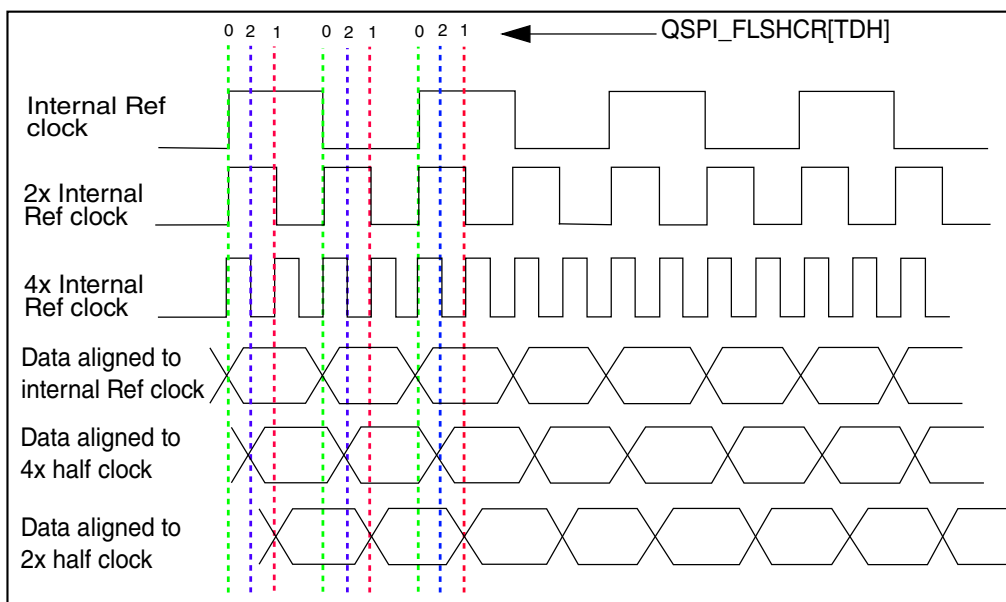
Figure 35-20. Data Hold
