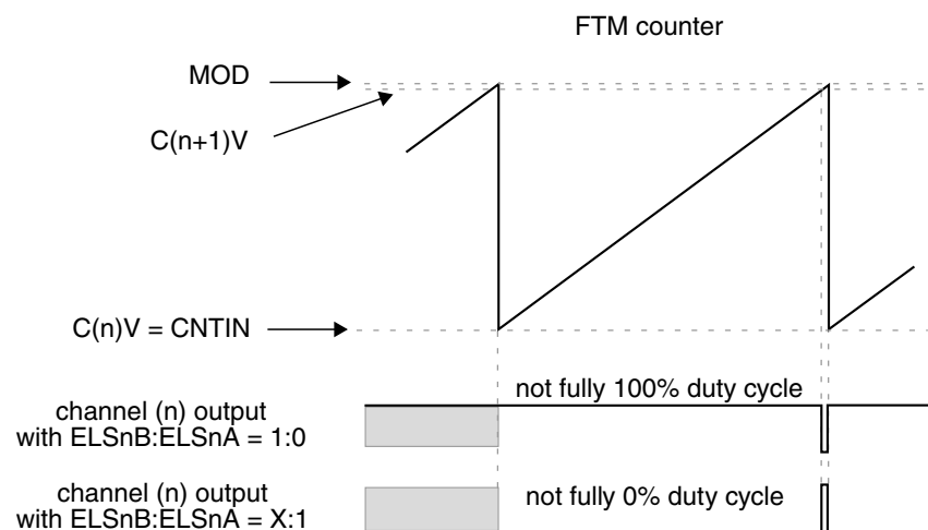
Figure 44-35. Channel (n) output if C(n)V = \text{CNTIN} and \text{CNTIN} < C(n+1)V < \text{MOD} and C(n+1)V is Almost Equal to MOD)
