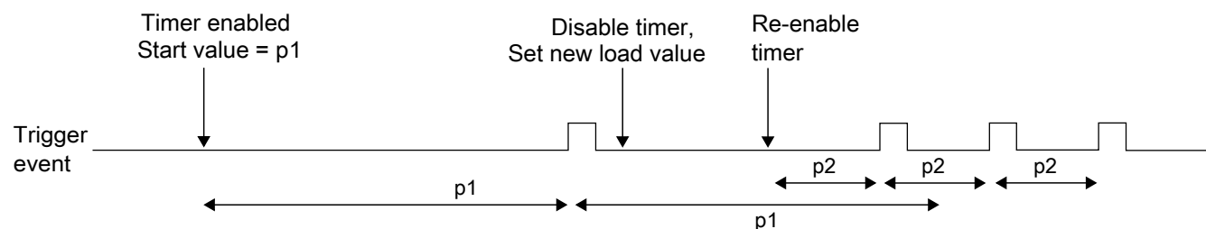
Figure 49-3. Modifying running timer period
