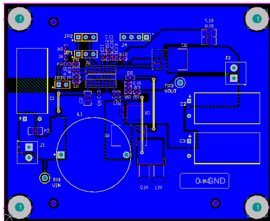
Figure 4. Assembly Layer
