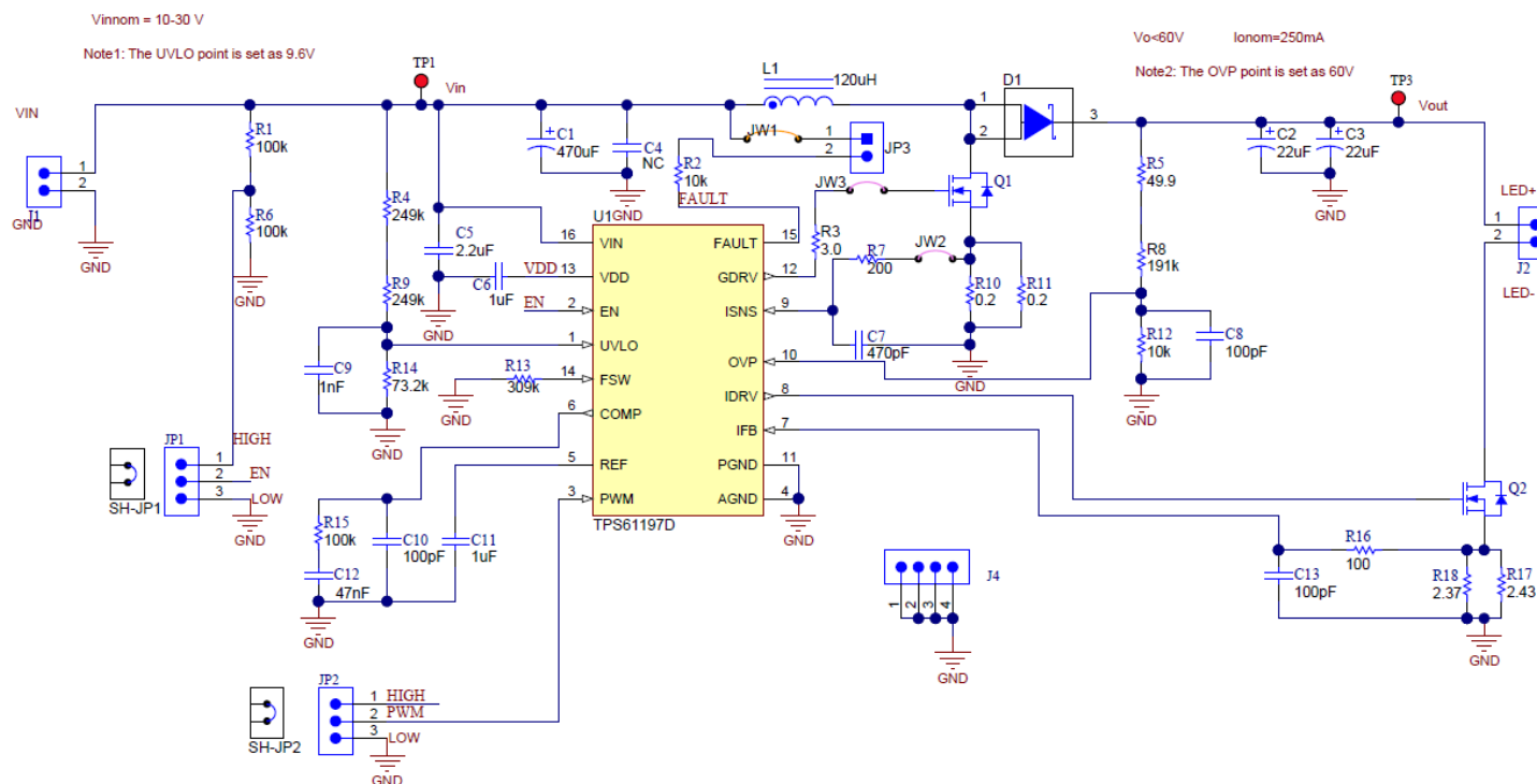
Figure 6. TPS61197EVM Schematic
