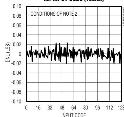
VARIABLE-RESISTOR DNL vs. INPUT CODE (100kΩ)
