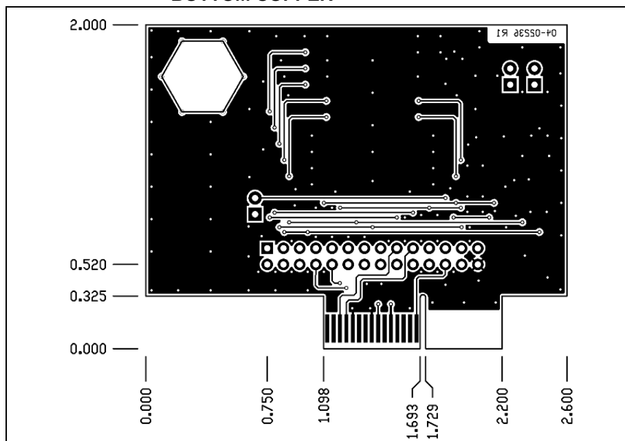
FIGURE A-4: MRF24J40MC PICTail™/PICTail PLUS DAUGHTER BOARD BOTTOM COPPER
