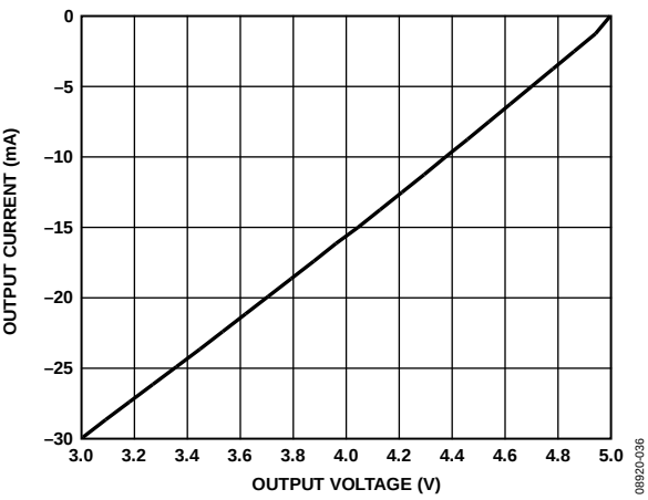
Figure 15. Output Current vs. Receiver Output High Voltage
