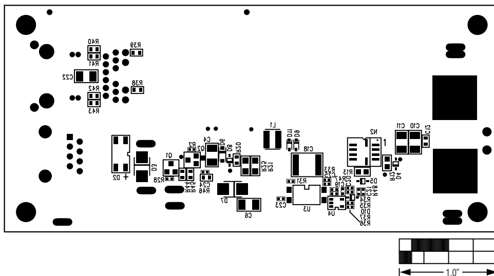
Component Placement Guide—Solder Side
