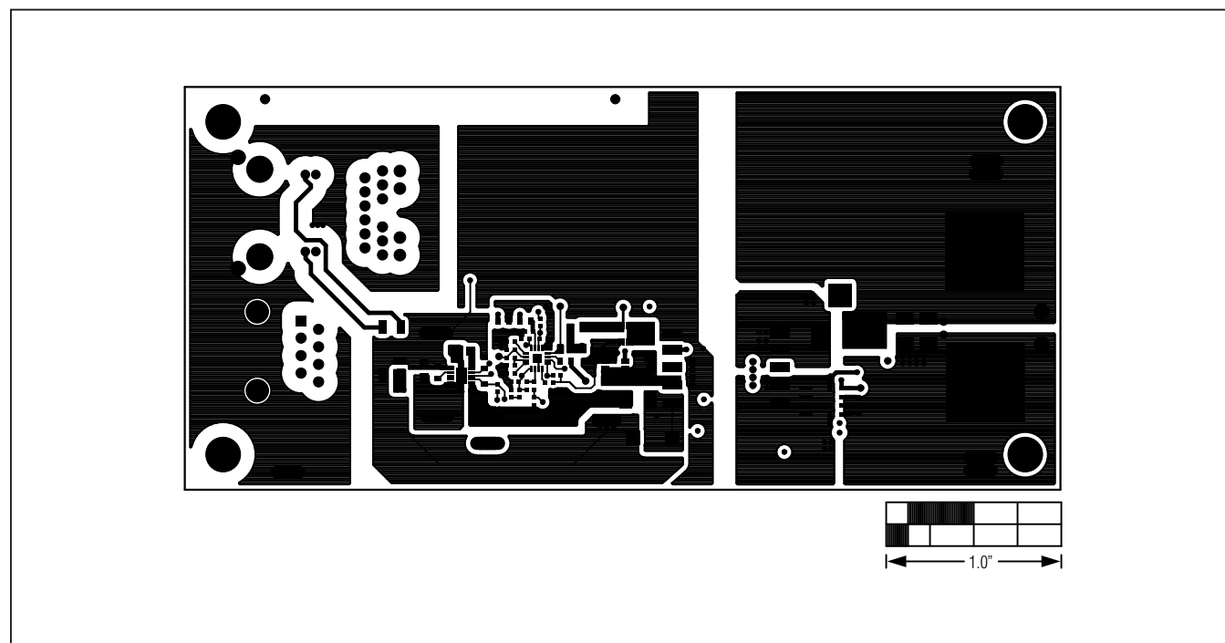
Component Side
