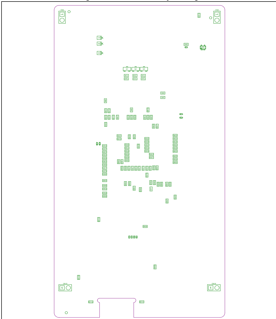
Figure 20. Bottom assembly drawing
