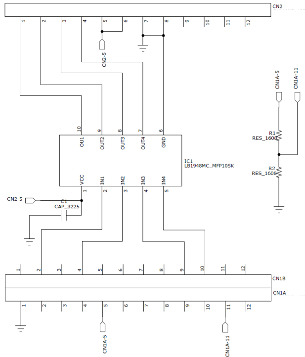
LV8548MCSLDGEVB Schematic
