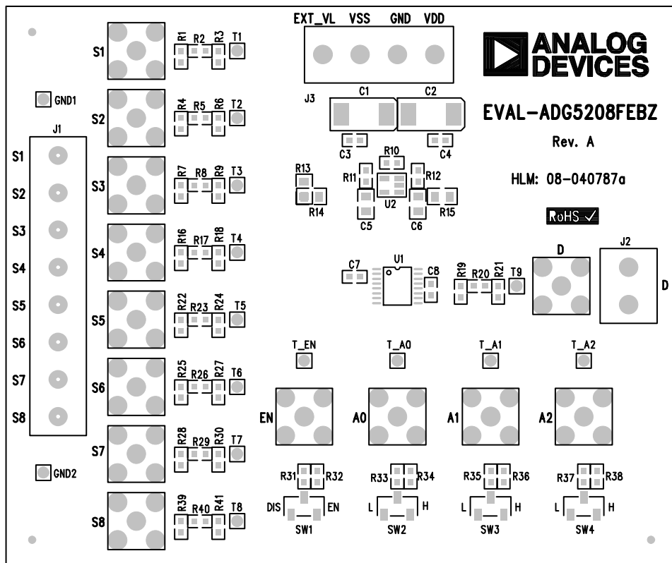
Figure 6. EVAL-ADG5208FEBZ Silkscreen
