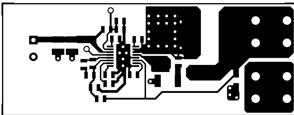
Figure 5. Component Side
