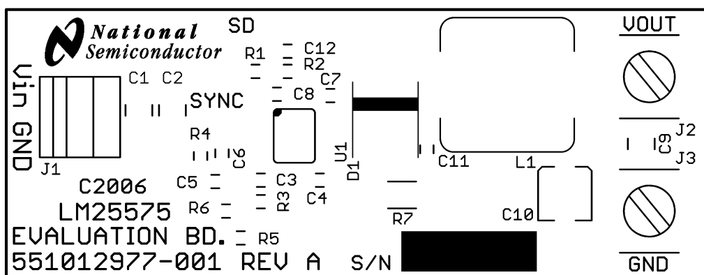
Figure 7. Silkscreen
