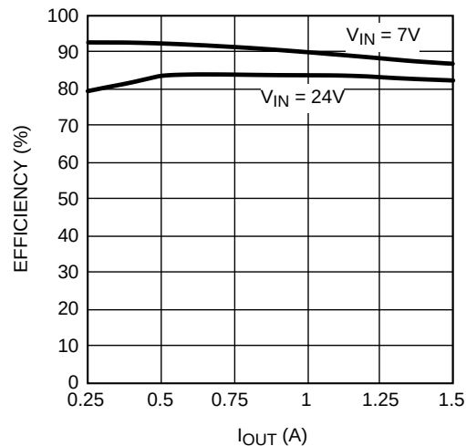
Figure 2. Conversion Efficiency vs Output Current
