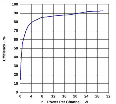
Figure 8. Efficiency Four Channels AT 4 Ω Each
