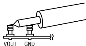
Figure 4. Measure Output Ripple
