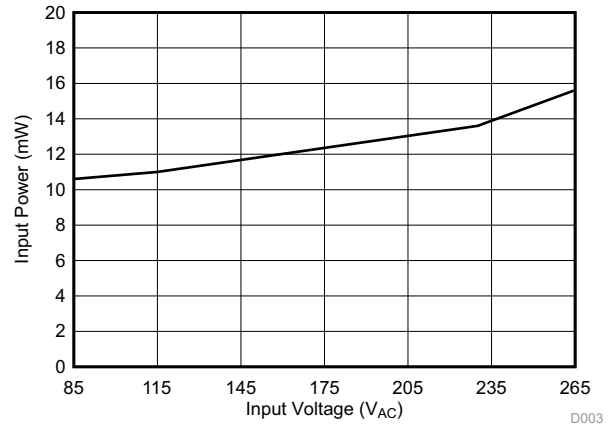
Figure 25. No Load Power Consumption
