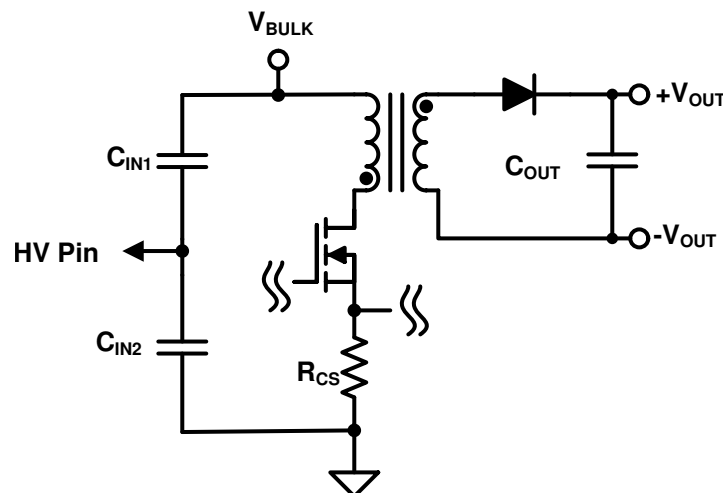
Figure 18. Implementation to Support > 700 V Inputs
