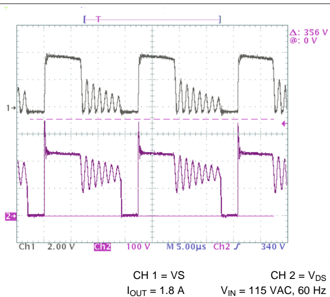
Figure 21. Switching Waveform
