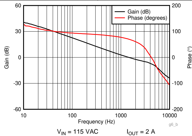
Figure 28. Bode Plot
