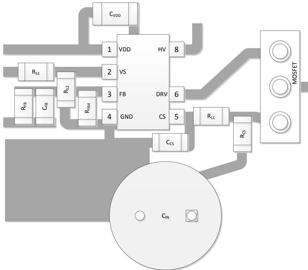
Figure 29. Layout Example Schematic
