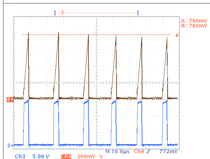
Figure 22. EMI Dithering
