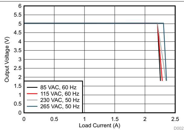
Figure 26. V OUT vs. I OUT
