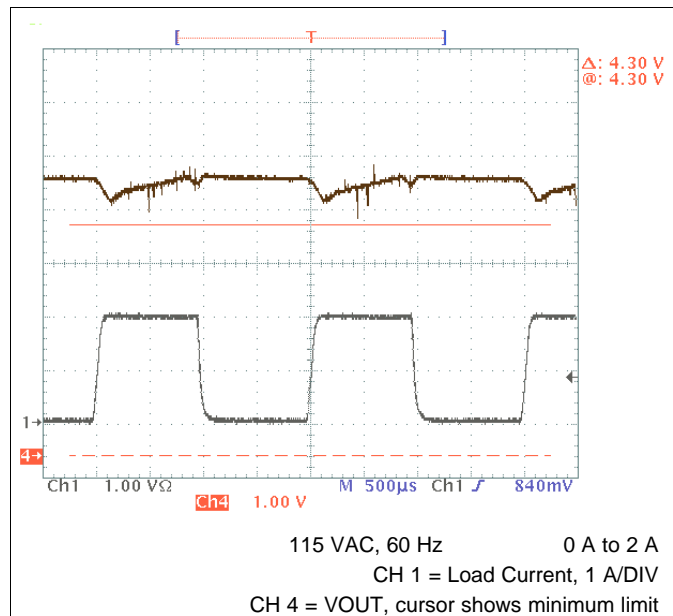
Figure 20. Transient Response
