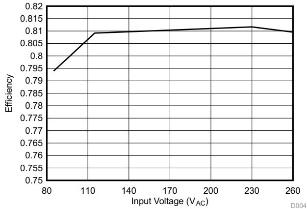
Figure 24. Average Efficiency
