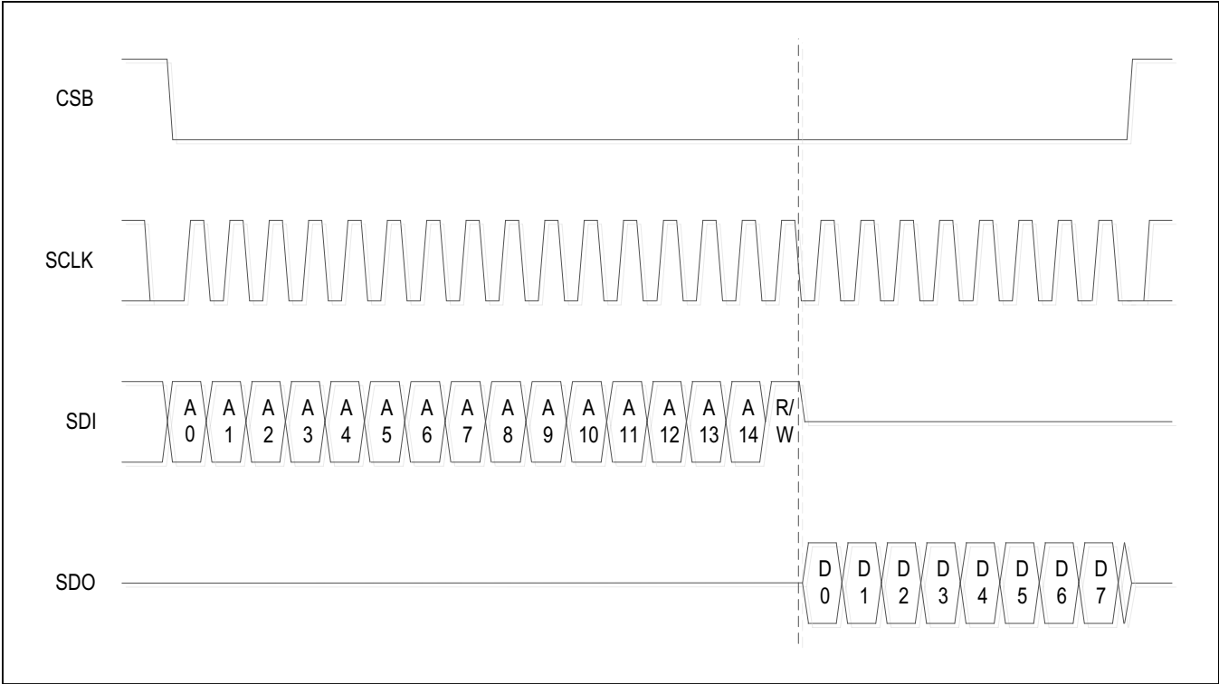
Figure 15. Single SPI Read Transaction with LSB-First
