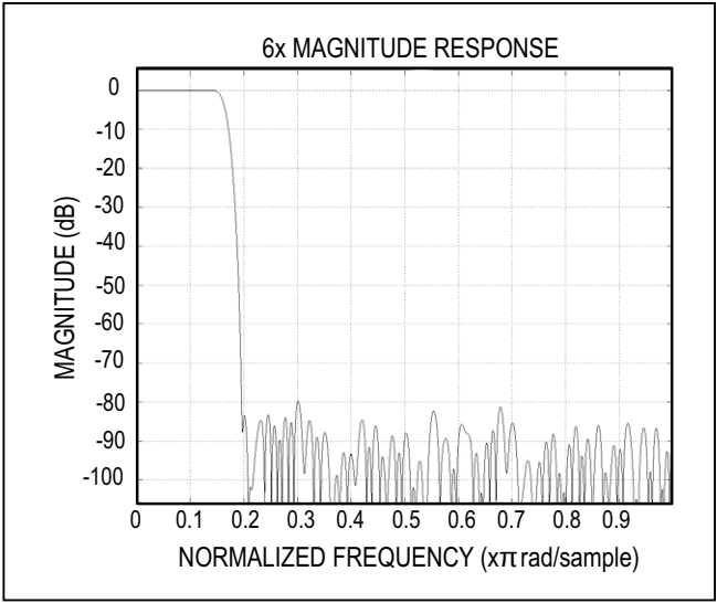
Figure 31. 6x Filter Baseband Frequency Response Normalized to DAC Output Update Rate
