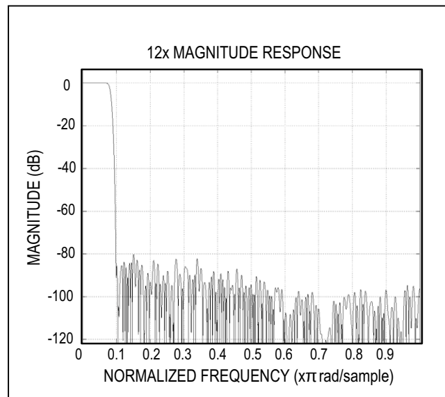
Figure 35. 12x Filter Baseband Frequency Response Normalized to DAC Output Update Rate
