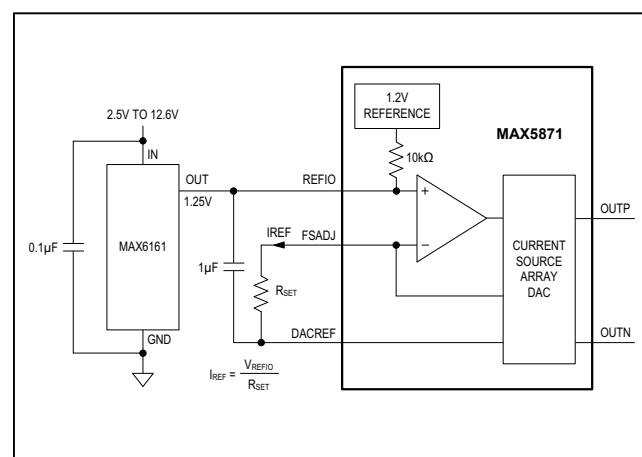
Figure 25b. Reference Architecture, External Reference Configuration
