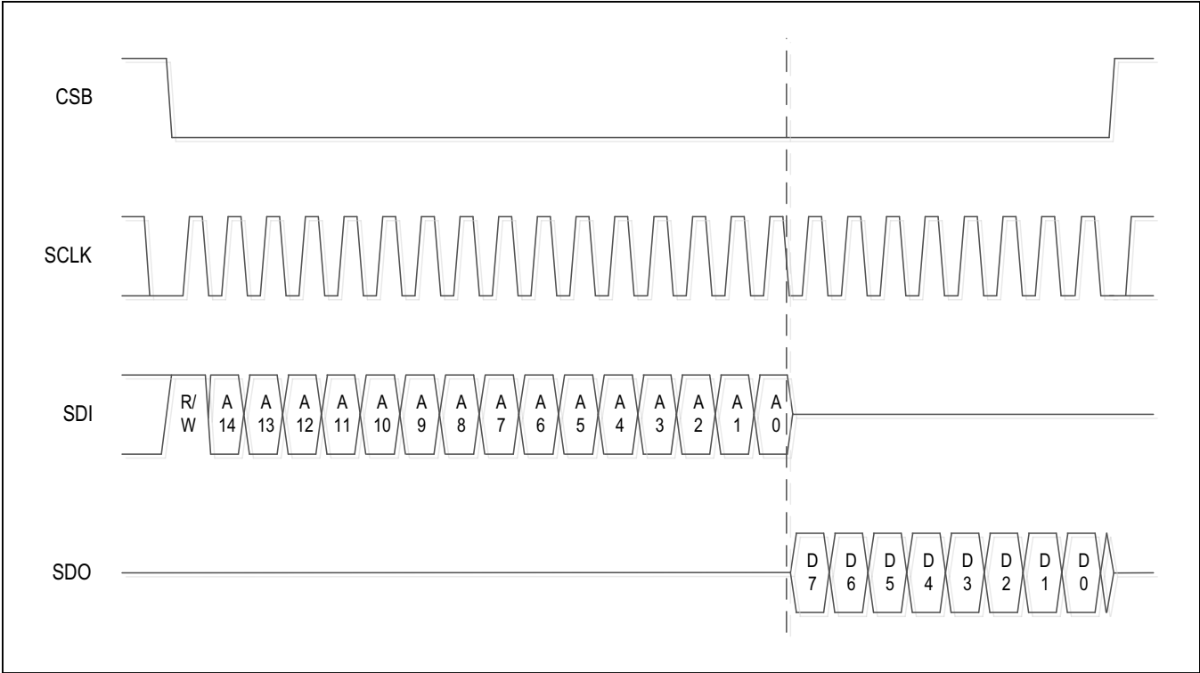
Figure 13. Single SPI Read Transaction with MSB-First
