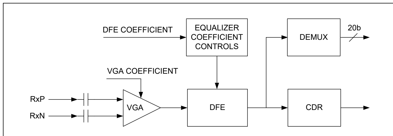
Figure 2. JESD204B Rx Physical Layer Simplified Block Diagram
