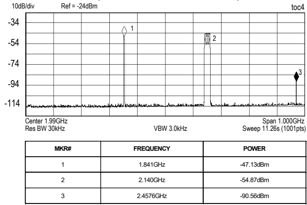
SIX-CARRIER GSM ( f_{OUT} = 1.8425GHz ) and 4-CARRIER WCDMA ( f_{OUT} = 2.14GHz ), WIDE-BAND SPECTRUM (INPUT AMPLITUDE = -1dBFS)
