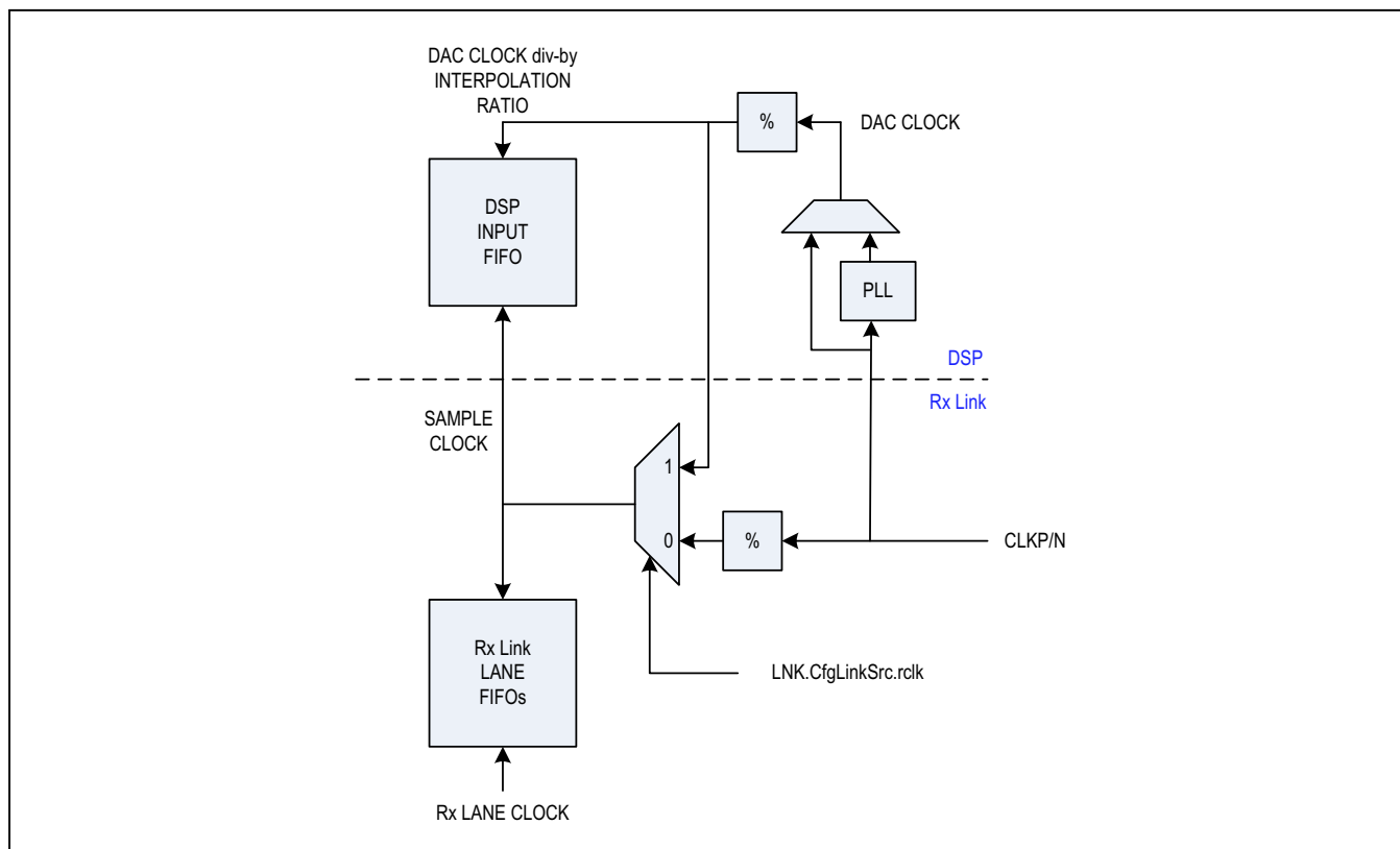
Figure 40. Rx Link and DSP Clocking
