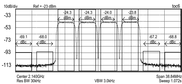
SIX-CARRIER GSM ( f_{OUT} = 1.8425GHz ) and 4-CARRIER WCDMA ( f_{OUT} = 2.14GHz ), NARROW-BAND WCDMA SPECTRUM (INPUT AMPLITUDE = -1dBFS)
