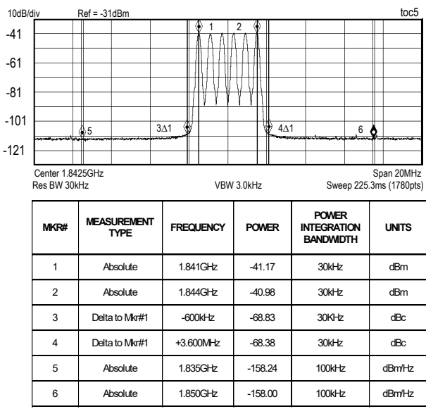
SIX-CARRIER GSM ( f_{OUT} = 1.8425GHz ) and 4-CARRIER WCDMA ( f_{OUT} = 2.14GHz ), NARROW-BAND GSM SPECTRUM (INPUT AMPLITUDE = -1dBFS)
