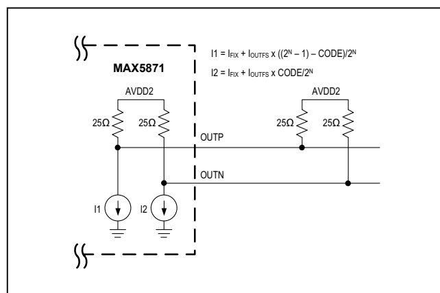
Figure 27. Output Configuration for Low-Frequency Operation
