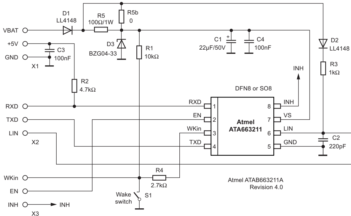
Figure 2-1. Schematic of the ATAB663211A Development Board
