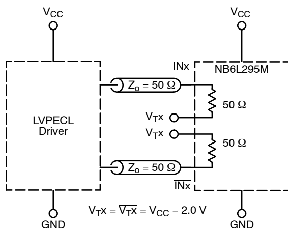
Figure 17. LVPECL Interface
