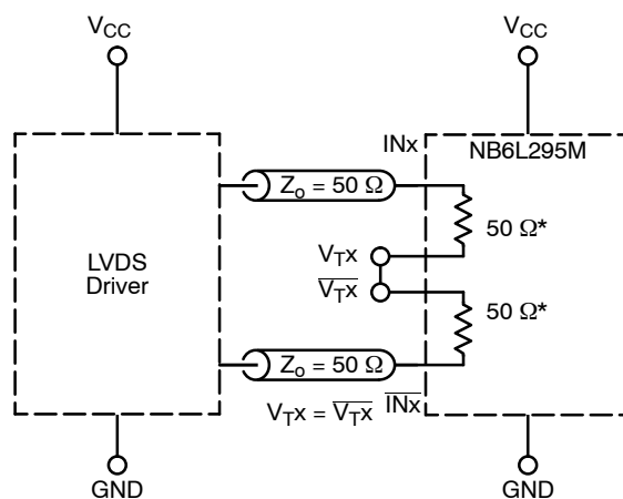
Figure 18. LVDS Interface
