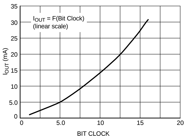
Figure 9. Typical Output Current Slope
