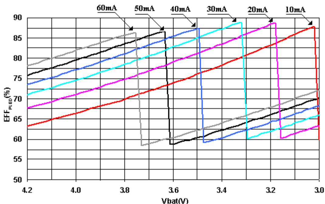
Figure 10. Typical Efficiency
