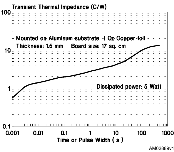
Figure 10. PowerSO20 transient thermal resistance
