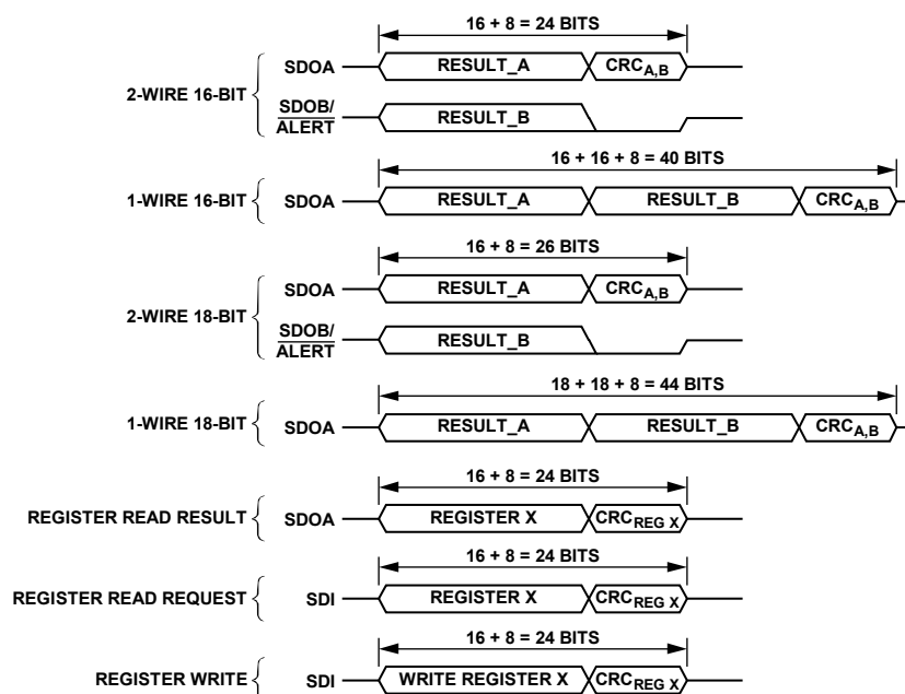
Figure 43. CRC Operation
