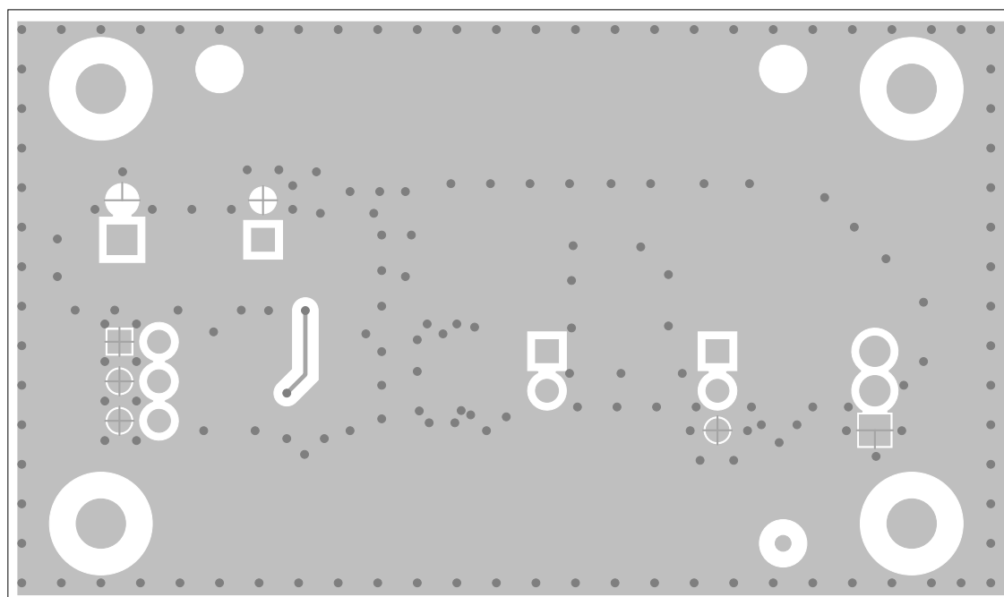
Figure 3. Bottom Layer
