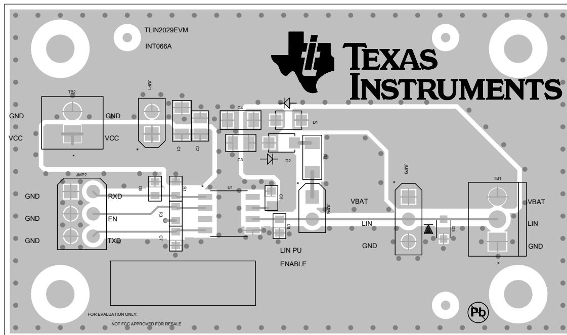
Figure 2. Top Layer
