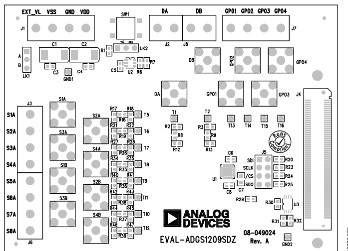
Figure 20. EVAL-ADGS1209SDZ Silk Screen
