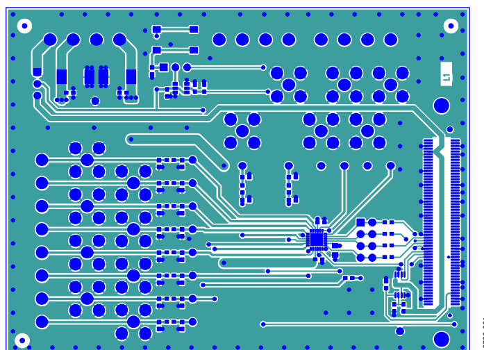
Figure 21. EVAL-ADGS1209SDZ Top Layer
