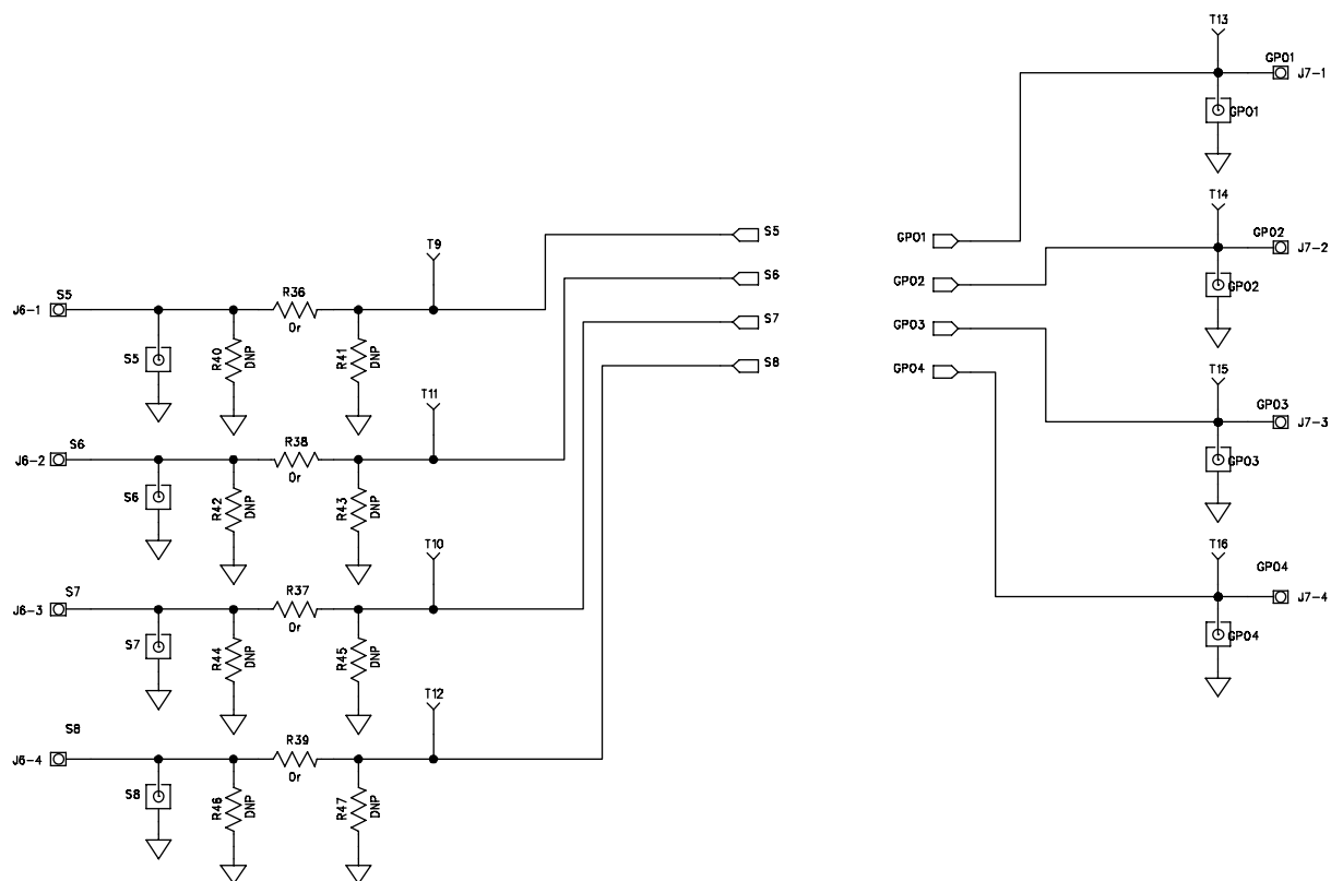
Figure 8. EVAL-ADGS1208SDZ Schematic 2
