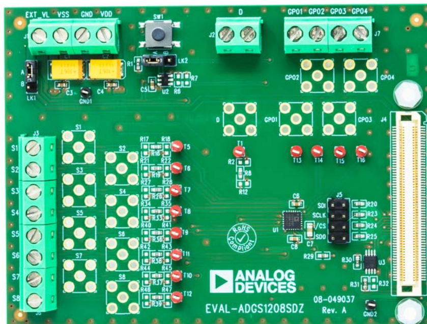
Figure 1. EVAL-ADGS1208SDZ
