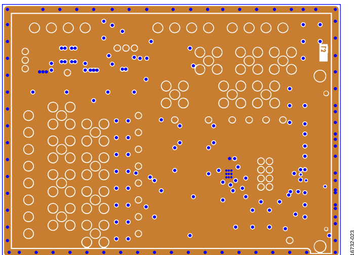
Figure 23. EVAL-ADGS1209SDZ Layer 3
