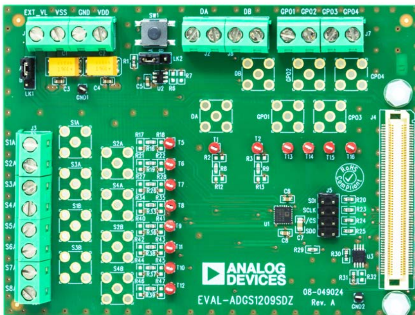
Figure 2. EVAL-ADGS1209SDZ
