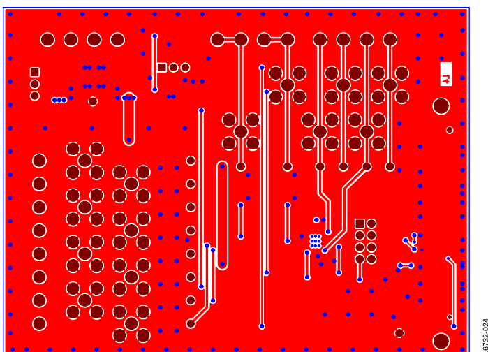
Figure 24. EVAL-ADGS1209SDZ Bottom Layer
