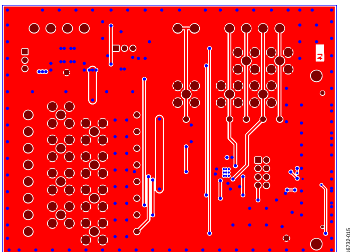
Figure 15. EVAL-ADGS1208SDZ Bottom Layer
