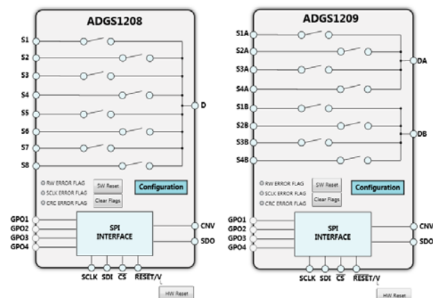
Figure 3. Evaluation Board View of the EVAL-ADGS1208SDZ/EVAL-ADGS1209SDZ
