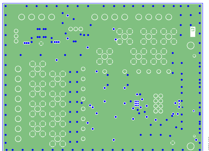
Figure 22. EVAL-ADGS1209SDZ Layer 2
