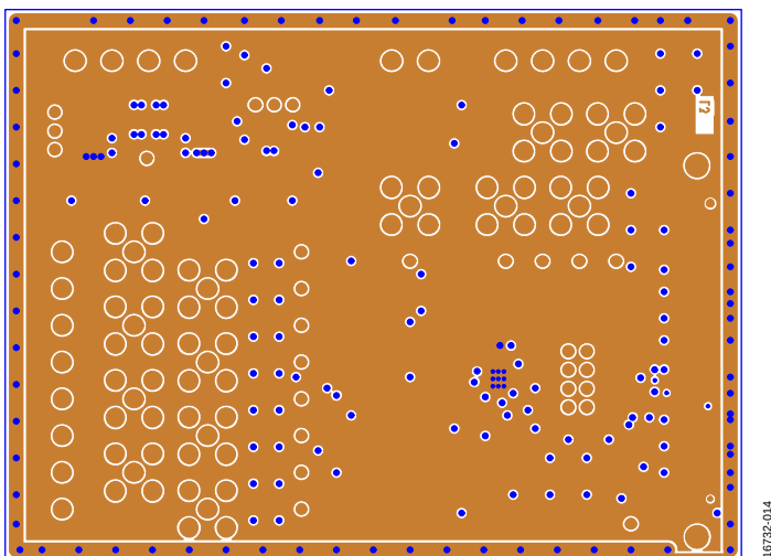
Figure 14. EVAL-ADGS1208SDZ Layer 3
