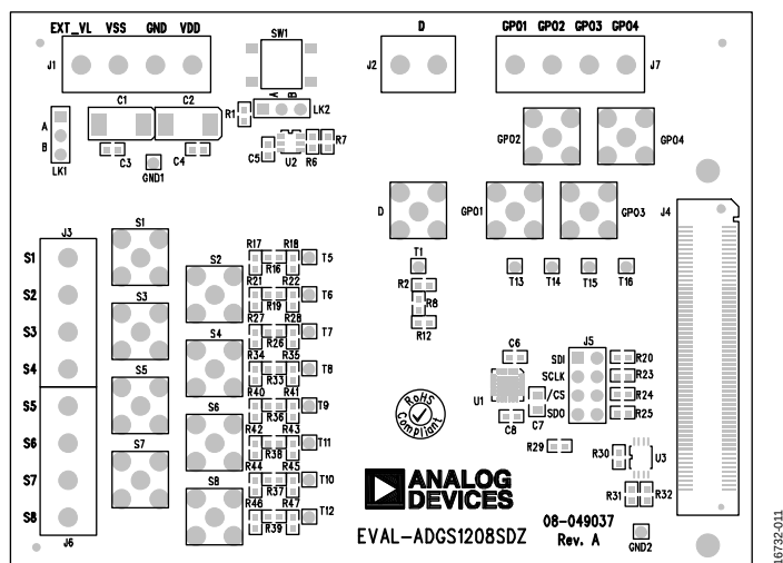
Figure 11. EVAL-ADGS1208SDZ Silk Screen
