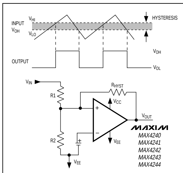
Figure 10. Hysteresis Comparator Circuit
