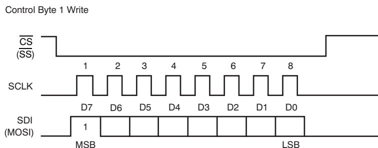
Figure 28. Interface Timing — Control Byte 1
