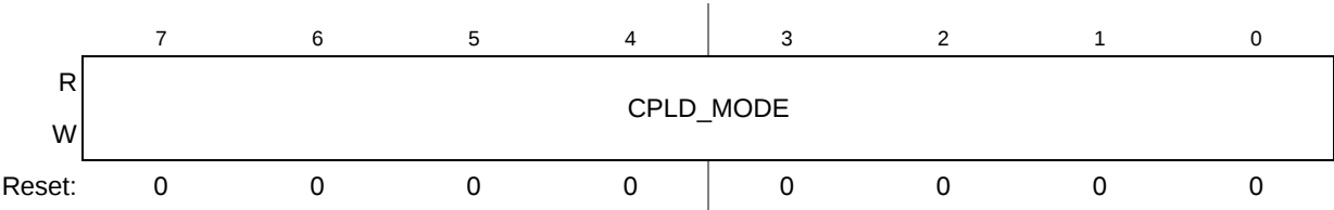
Figure 22. CPLD_MODE Register
