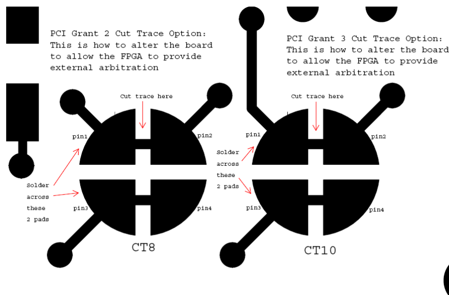
Figure 11. PCI Grant 2 and Grant 3 Cut Trace Option—Use FPGA for Arbitration
