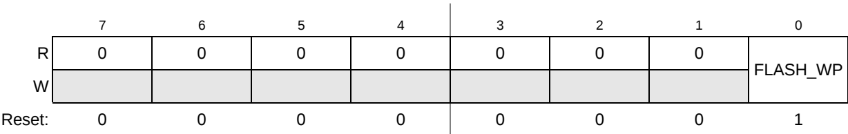
Figure 23. CPLD_FLASHCFG Register
