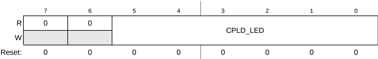
Figure 24. CPLD_LEDS Register
