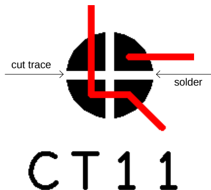
Figure 5. MCF5445x Input Clock Selection Cut-Trace
