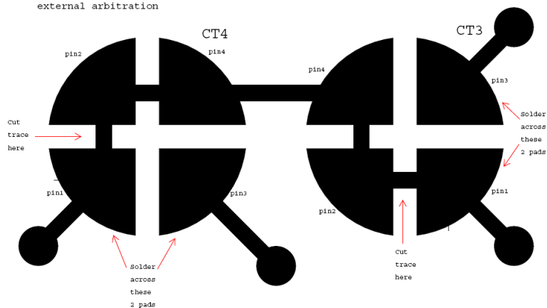
Figure 9. PCI Grant 0 Cut Trace Option—Use FPGA for Arbitration
