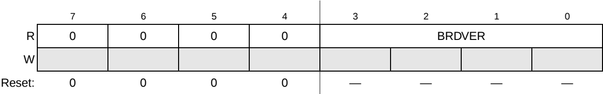
Figure 19. CPLD_VERSION Register
