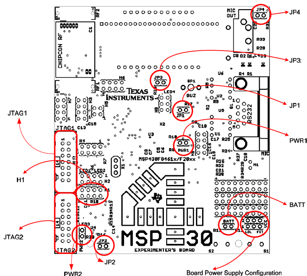
Figure 6. Jumper Locations
