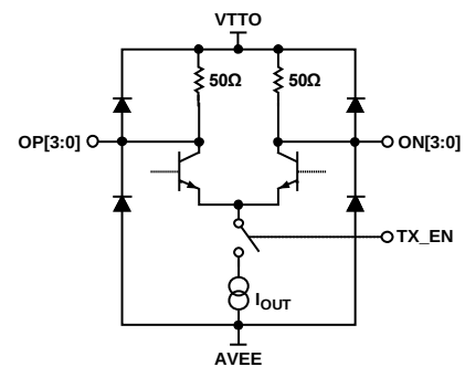
Figure 26. High Speed Output Simplified Schematic
