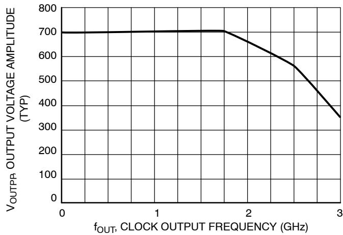
Figure 5. Output Voltage Amplitude ( V_{\text{OUTPR}} ) versus Clock Output Frequency at Ambient Temperature (Typical)
