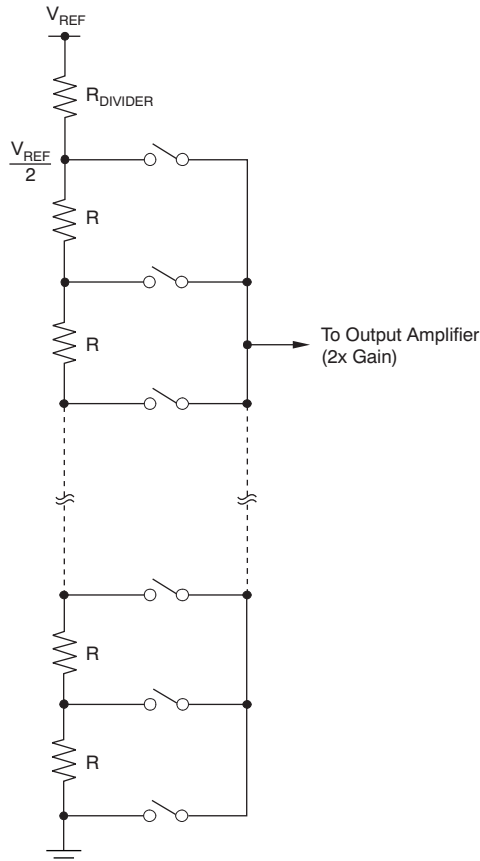
Figure 28. Resistor String
