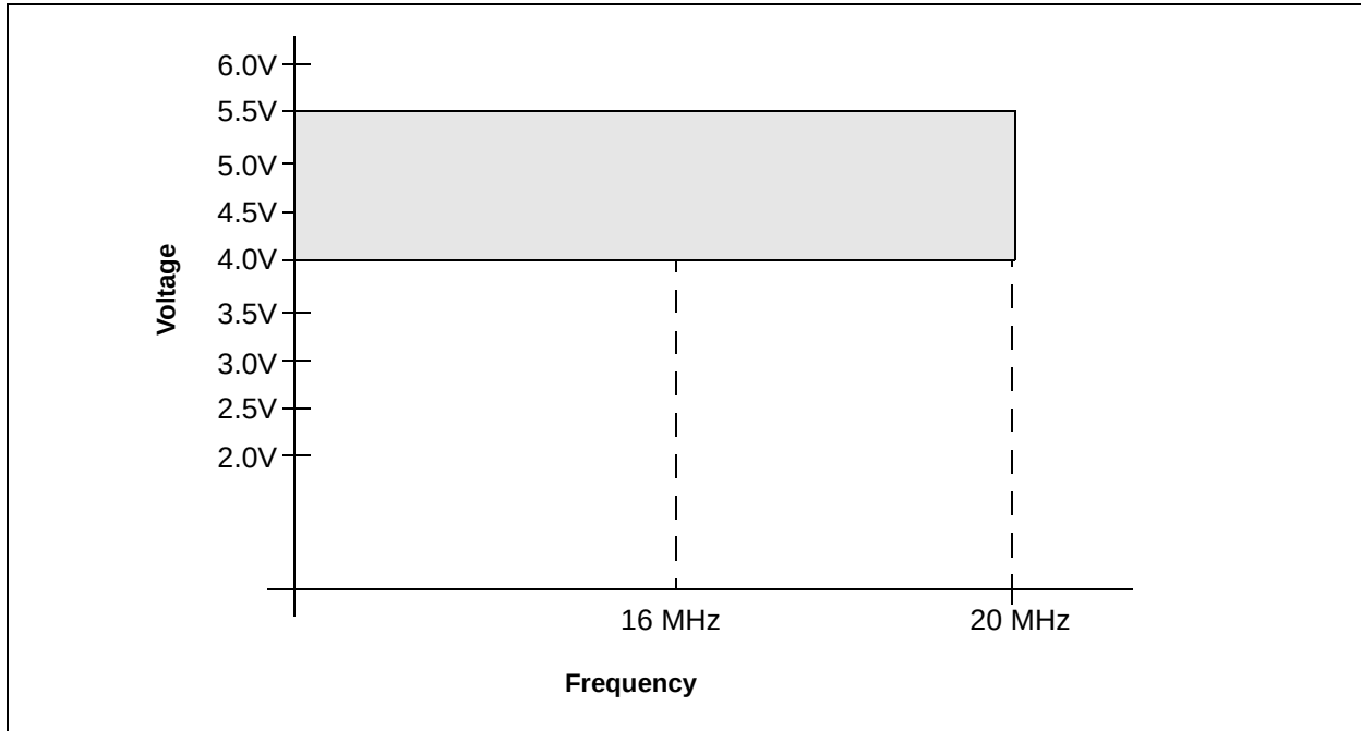
FIGURE 15-1: PIC16CR7X VOLTAGE-FREQUENCY GRAPH
