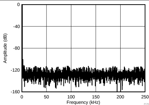
Figure 88. FFT Plot With a DC Common-Mode at 1 MSPS
