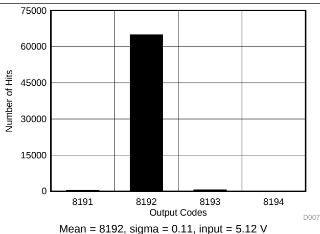
Figure 19. DC Histogram for Mid-Scale Inputs (0 V–10.24 V)
