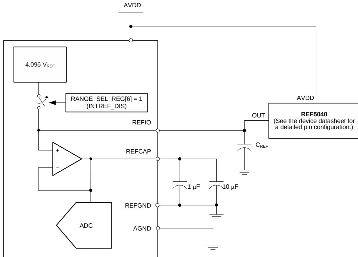
Figure 57. Device Connections for Using an External 4.096-V Reference
