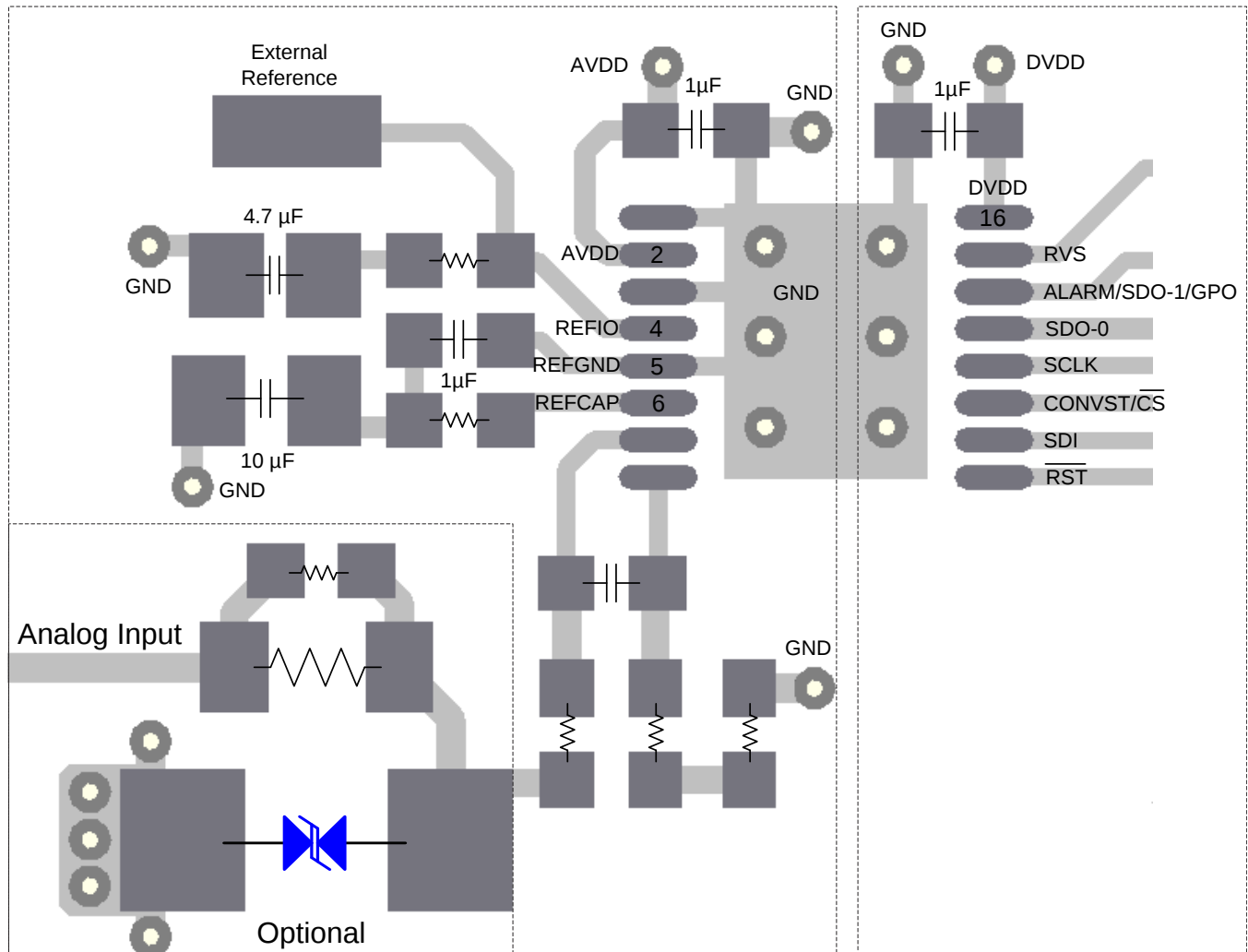
Figure 95. Board Layout for the ADS867x
