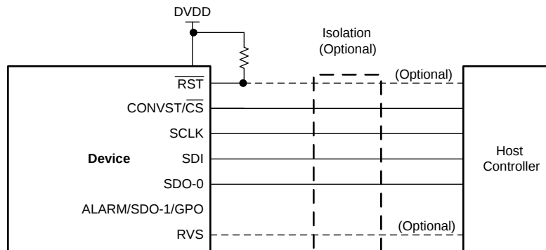
Figure 66. Standard SPI Protocol Pin Configuration
