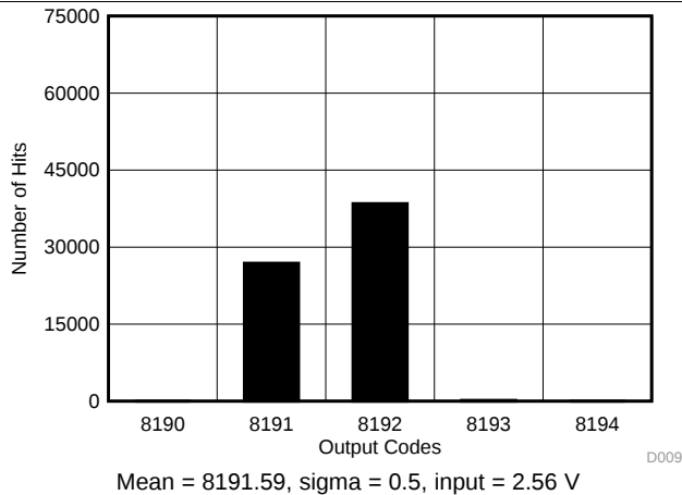
Figure 21. DC Histogram for Mid-Scale Inputs (0 V–5.12 V)
