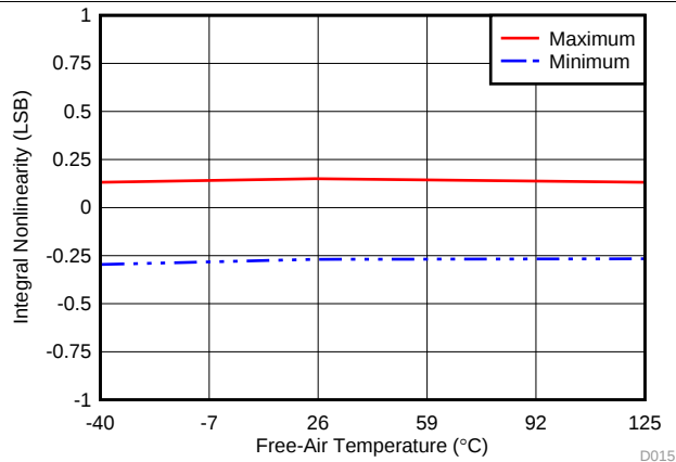
Figure 27. INL vs Temperature (All Unipolar Ranges)
