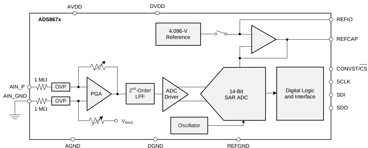
Block Diagram
