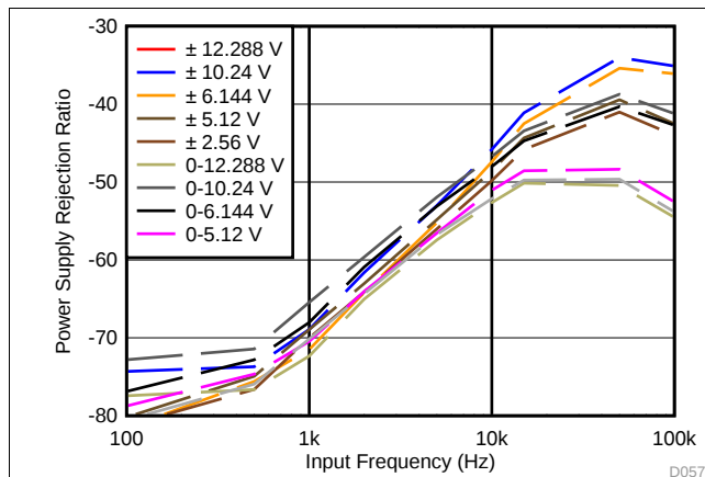
Figure 93. PSRR Without a Decoupling Capacitor
