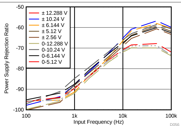
Figure 94. PSRR With a Decoupling Capacitor
