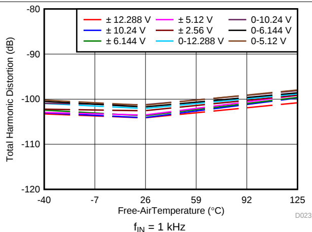
Figure 40. THD vs Temperature
