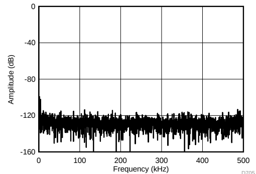
Figure 89. FFT Plot With an AC Common-Mode at 1 MSPS
