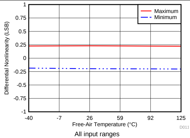
Figure 23. DNL vs Temperature
