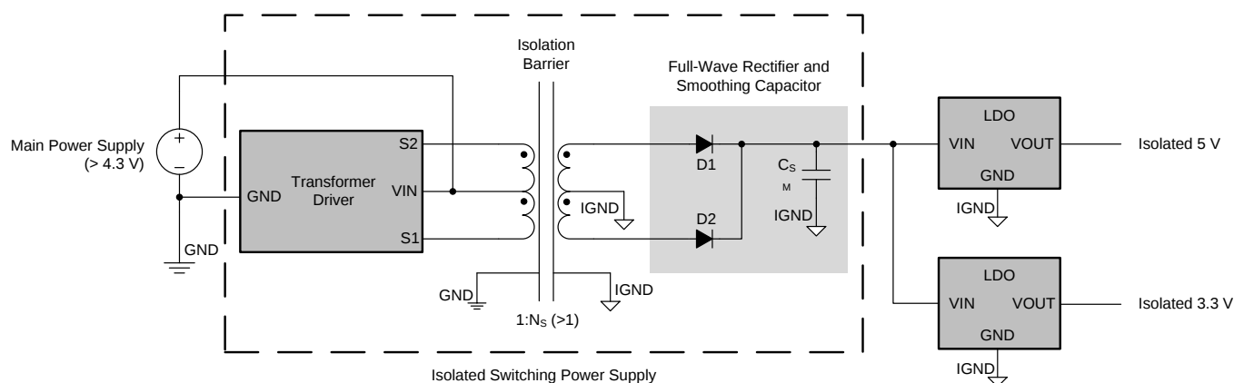
Figure 87. Isolated Power-Supply Design
