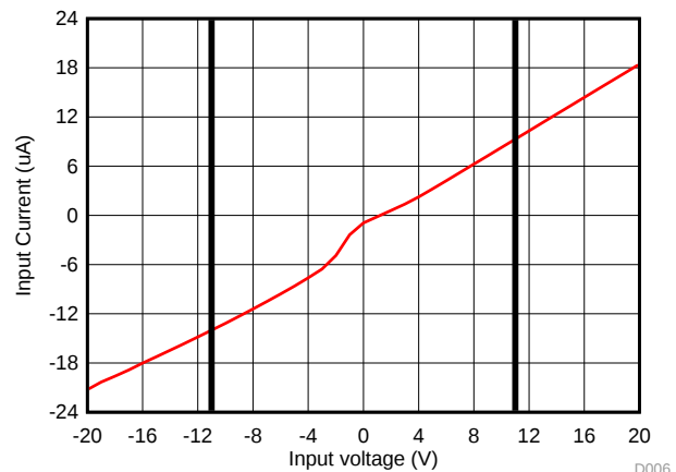
Figure 49. I-V Curve for the Input OVP Circuit (AVDD = Floating)
