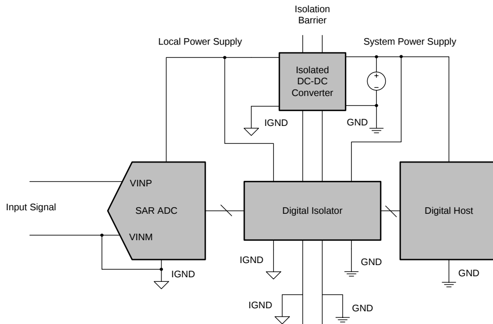
Figure 86. 14-Bit Isolated DAQ System for High Common-Mode Rejection
