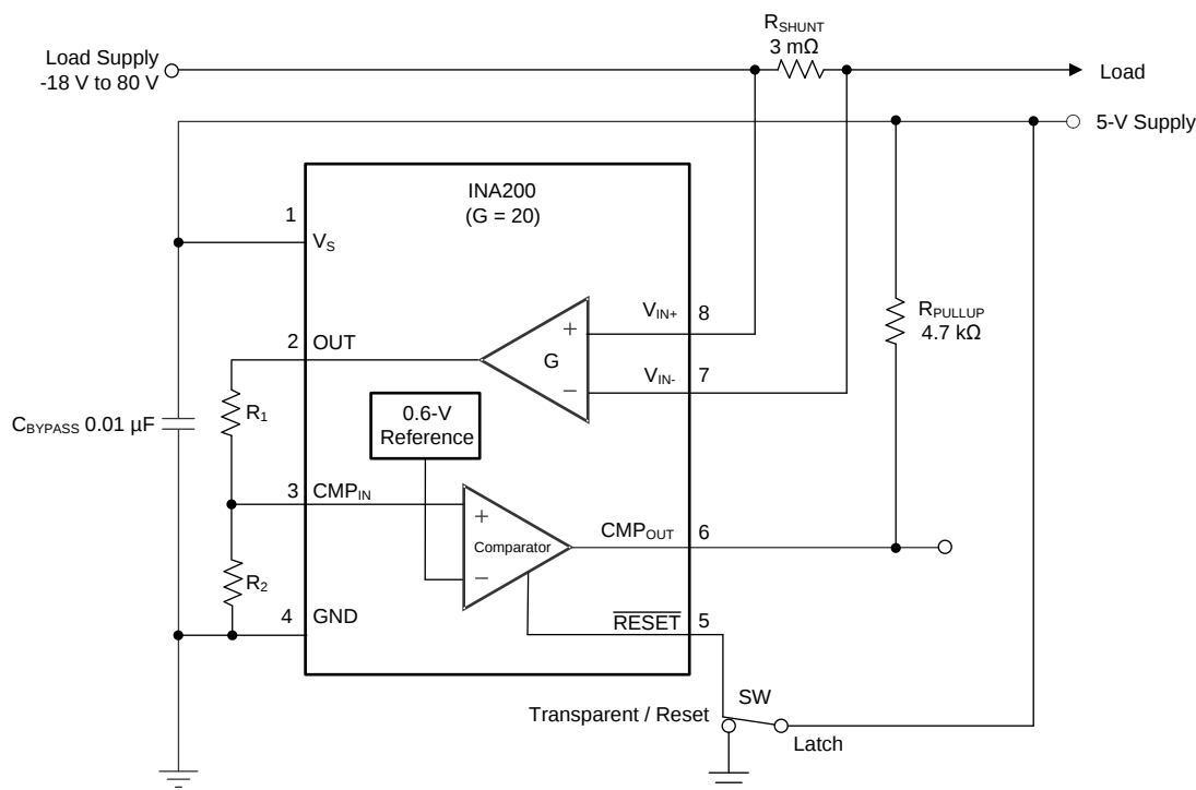
Figure 26. INA200 Basic Connections
