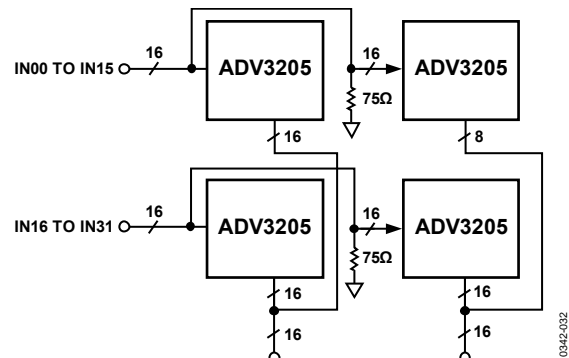
Figure 30. 32 × 32 Crosspoint Array Using Four ADV3205 Devices
