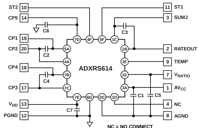
Figure 1. EVAL-ADXRS614 Schematic
