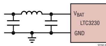
Figure 5. 10nH Inductor Used for Input Noise Reduction
